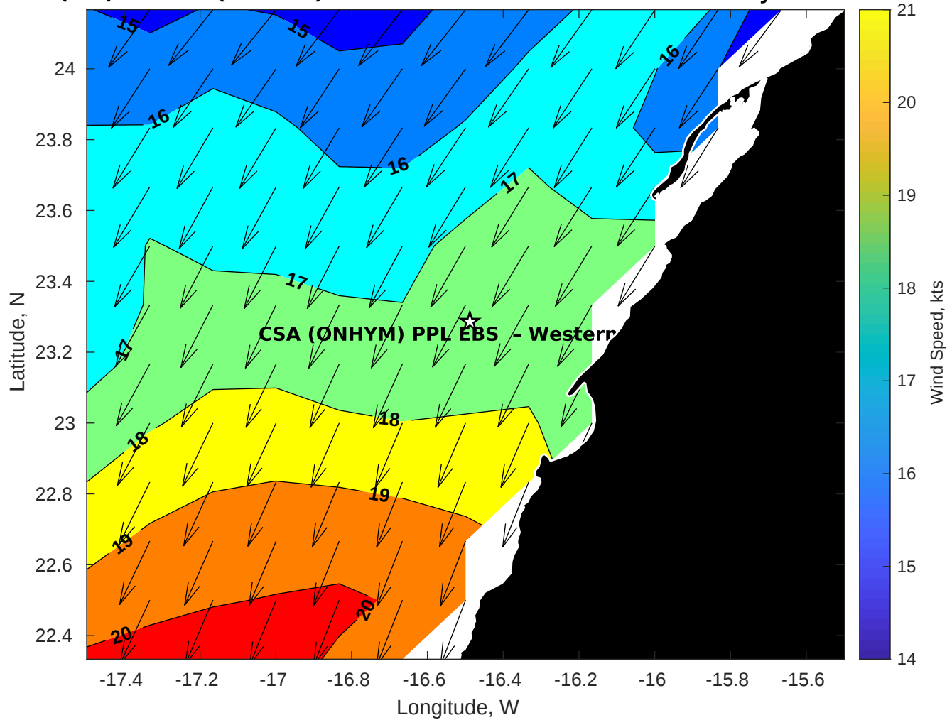
Winds (kts) for CSA (ONHYM) PPL EBS - Western Sahara at 18-May-2025 09:00:00
