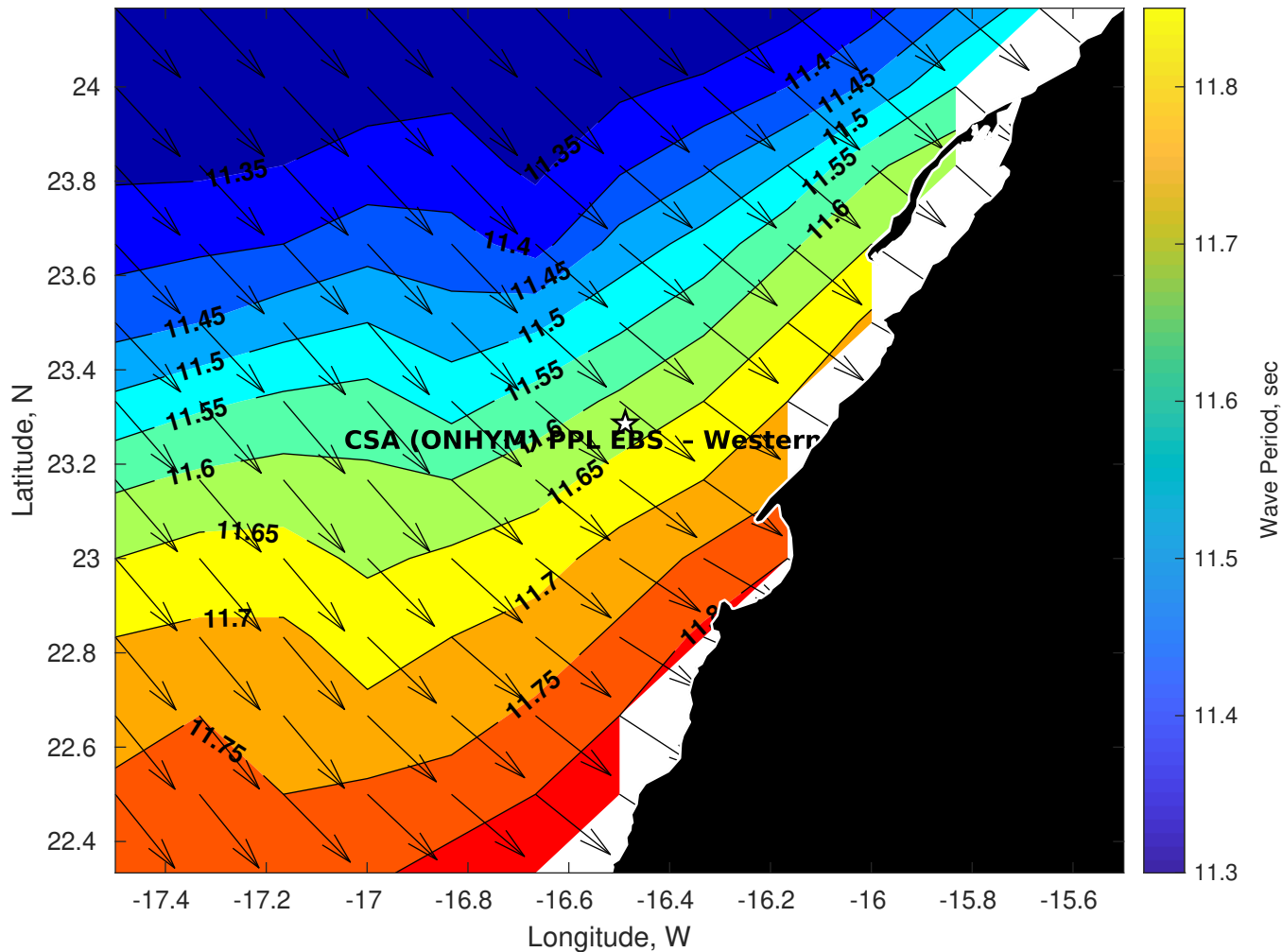
Wave Period (sec) for CSA (ONHYM) PPL EBS - Western Sahara at 18-May-2025 09:00:00
