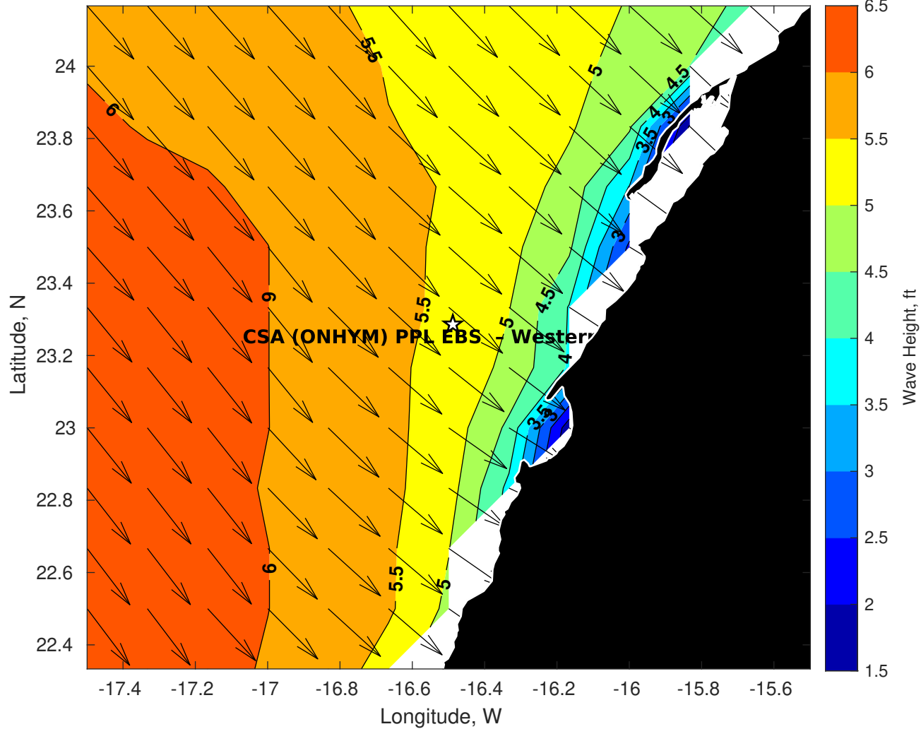
Wave Height (ft) for CSA (ONHYM) PPL EBS - Western Sahara at 18-May-2025 09:00:00
