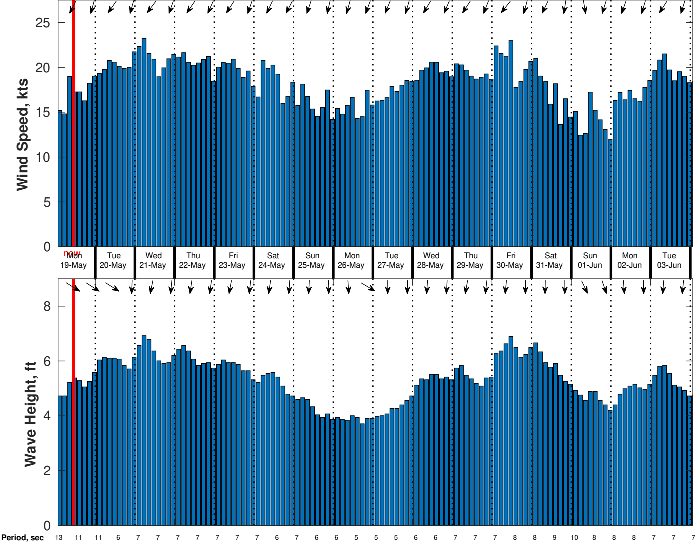
Wind & Wave Forecast for CSA (ONHYM) PPL EBS - Western Sahara from 18-May-2025 01:00:00 to 03-Jun-2025 01:00:00
