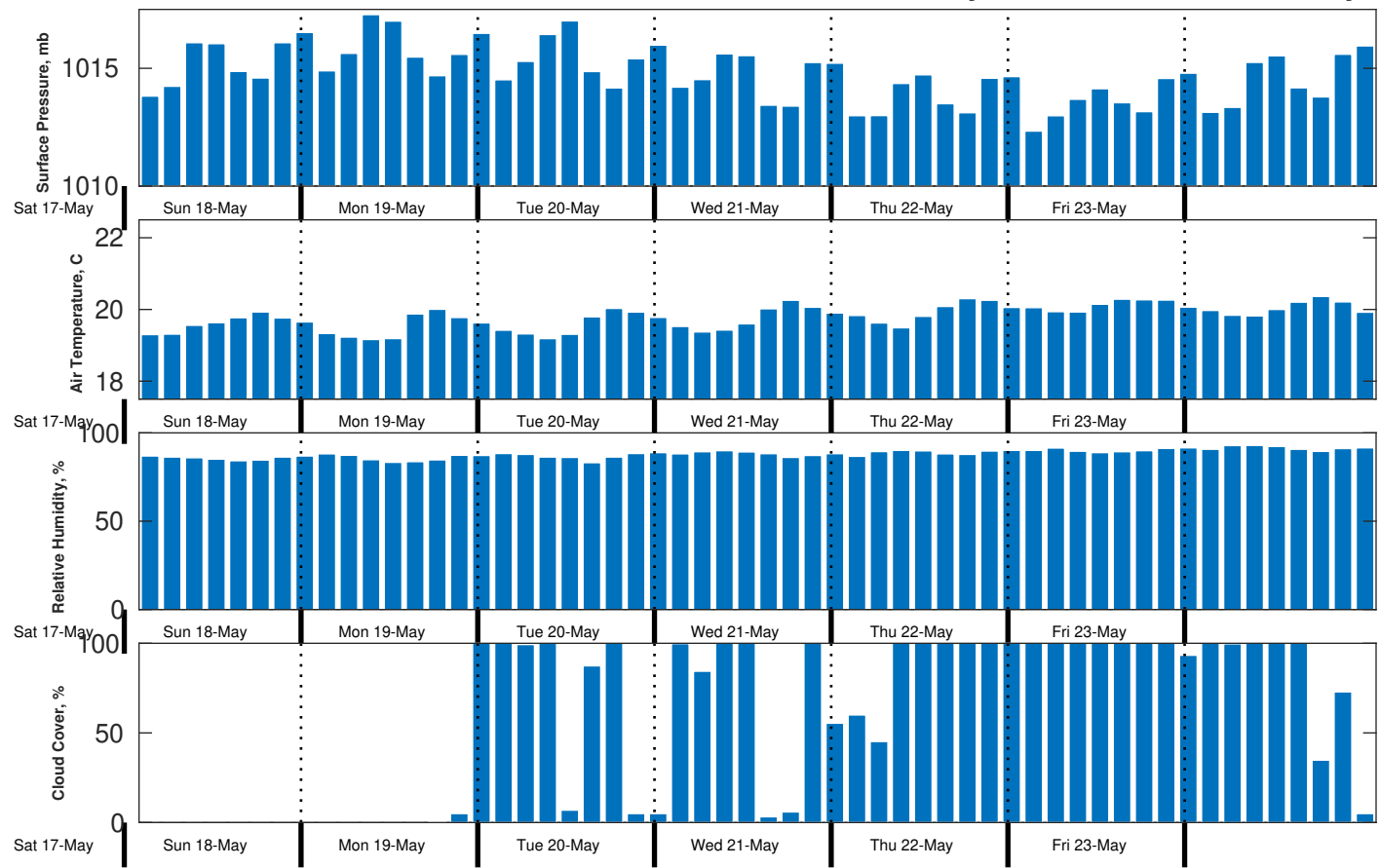
Met Forecast for CSA (ONHYM) PPL EBS - Western Sahara from 18-May-2025 00:00:00 to 25-May-2025 00:00:00
