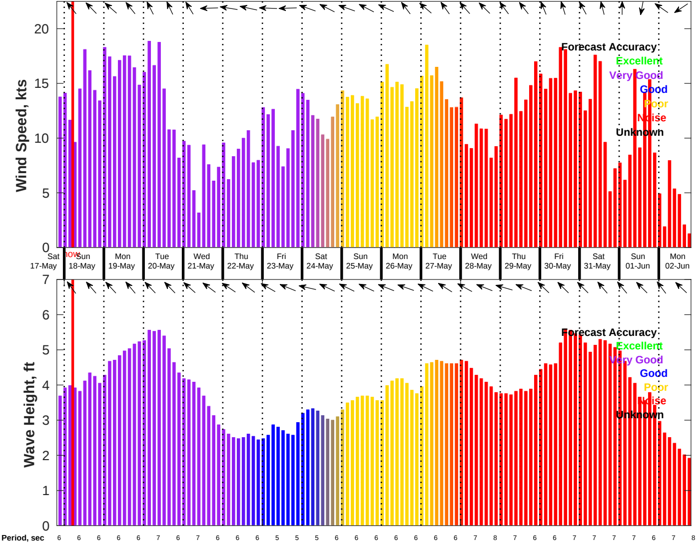
Wind & Wave Forecast for CTI Enbridge Kaskida & Tiber PPL Geotechnical from 17-May-2025 20:00:00 to 02-Jun-2025 20:00:00
