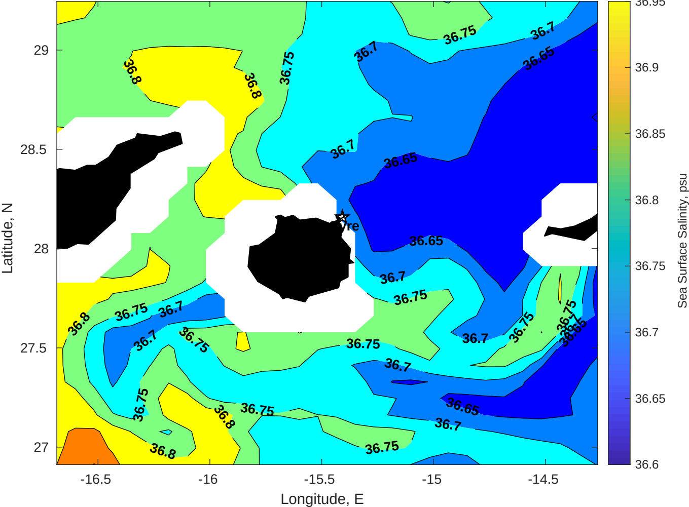
Surface Salinity for Gyre at 17-May-2025 00:00:00
