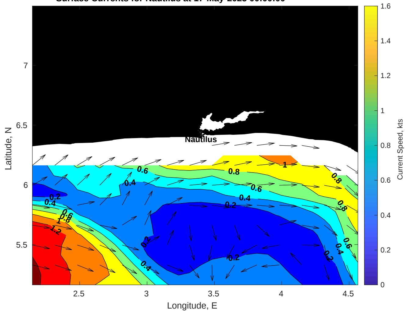
Surface Currents for Nautilus at 17-May-2025 00:00:00
