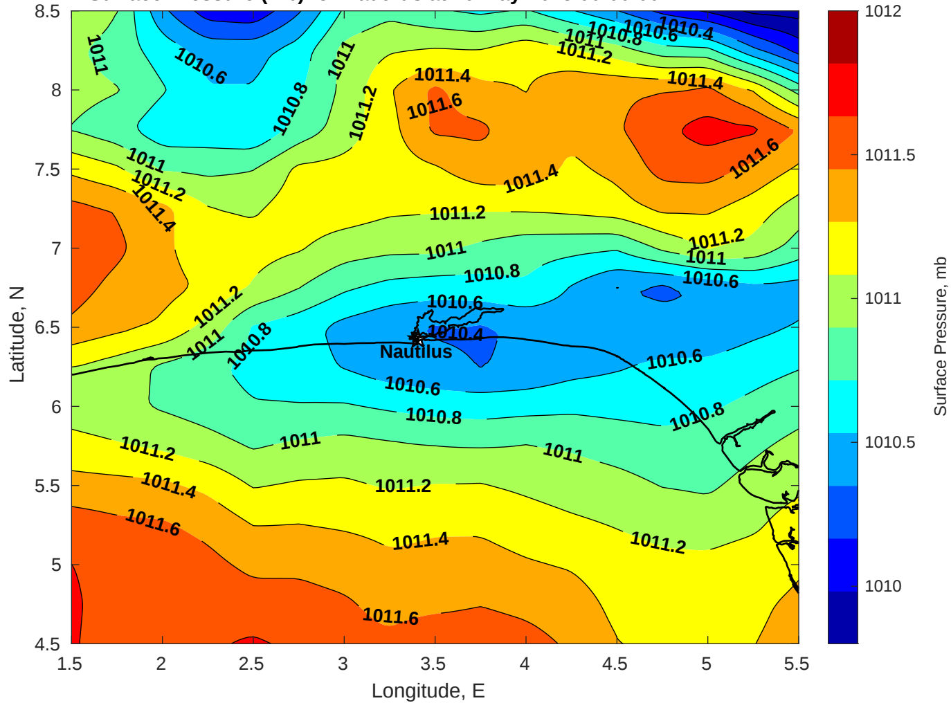
Surface Pressure (mb) for Nautilus at 20-May-2025 00:00:00
