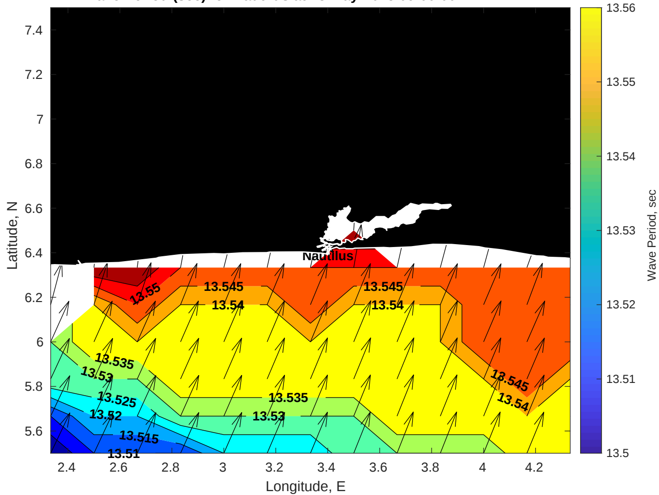
Wave Period (sec) for Nautilus at 18-May-2025 09:00:00
