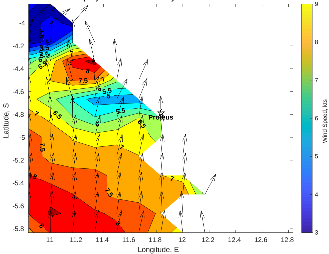
Winds (kts) for Proteus at 18-May-2025 09:00:00
