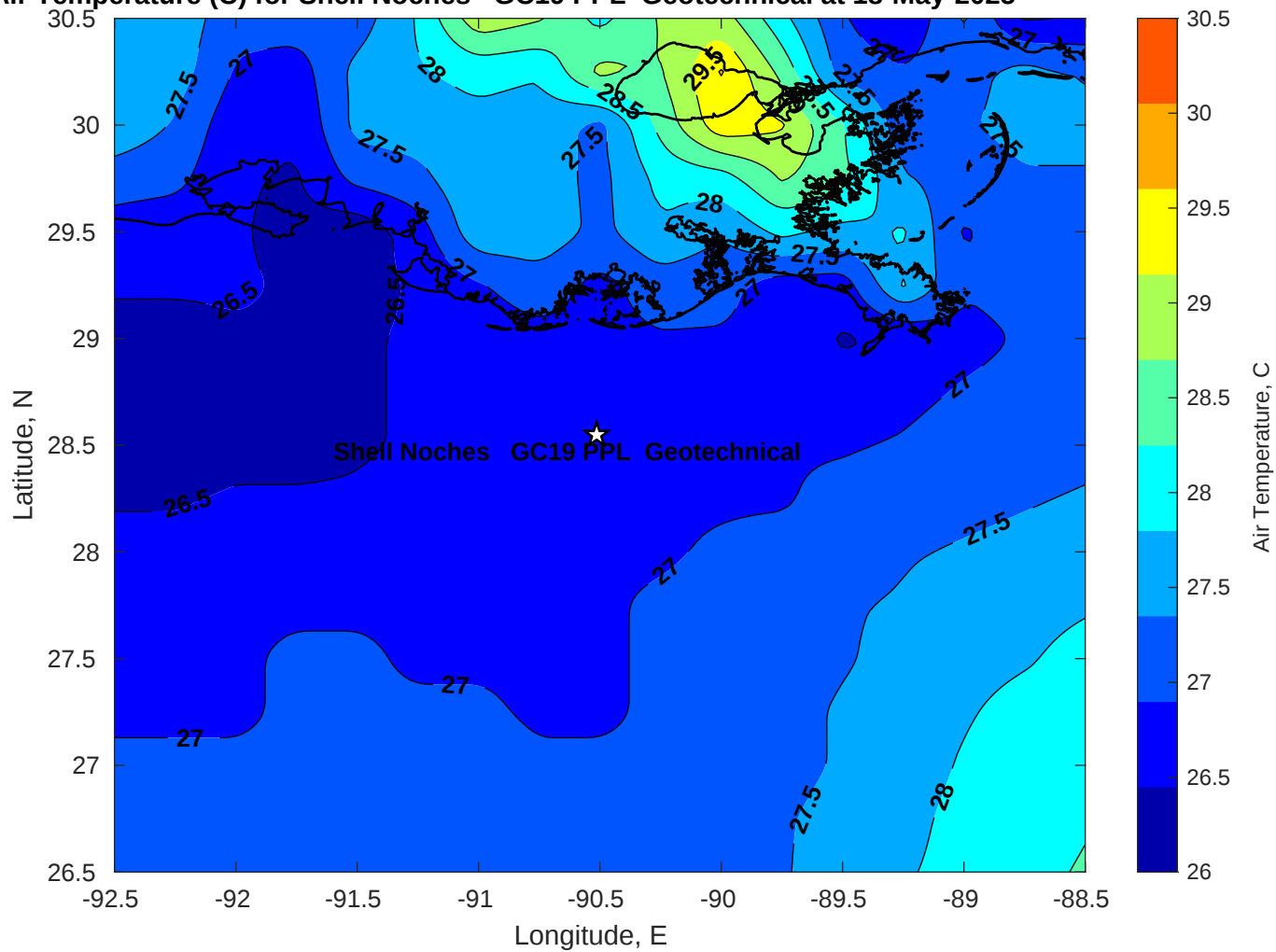
Air Temperature (C) for Shell Noches GC19 PPL Geotechnical at 18-May-2025
