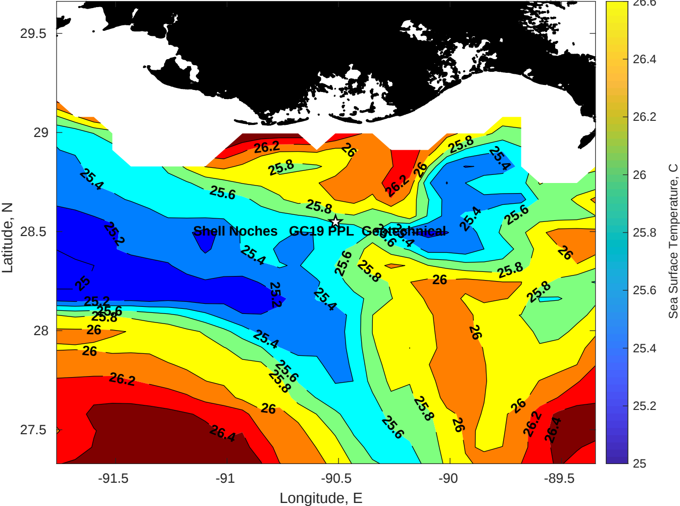
SST for Shell Noches GC19 PPL Geotechnical at 17-May-2025 00:00:00
