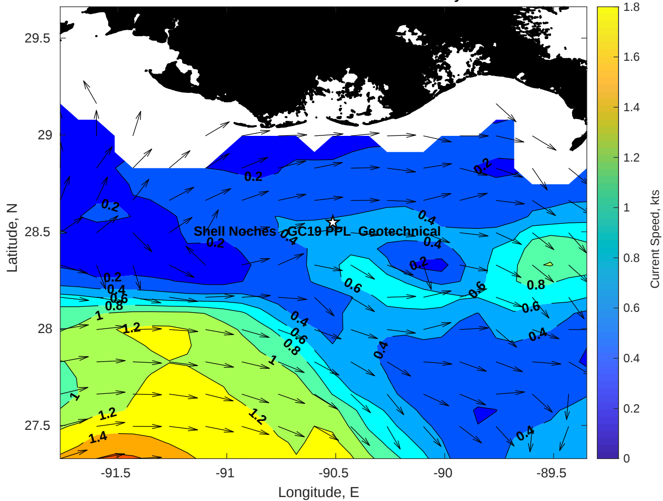
Surface Currents for Shell Noches GC19 PPL Geotechnical at 17-May-2025 00:00:00
