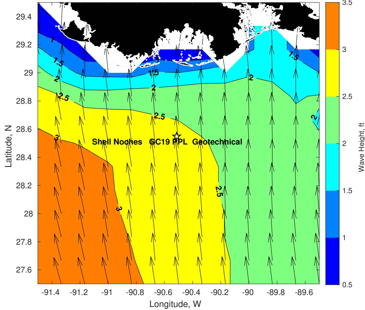
Wave Height (ft) for Shell Noches GC19 PPL Geotechnical at 18-May-2025 09:00:00
