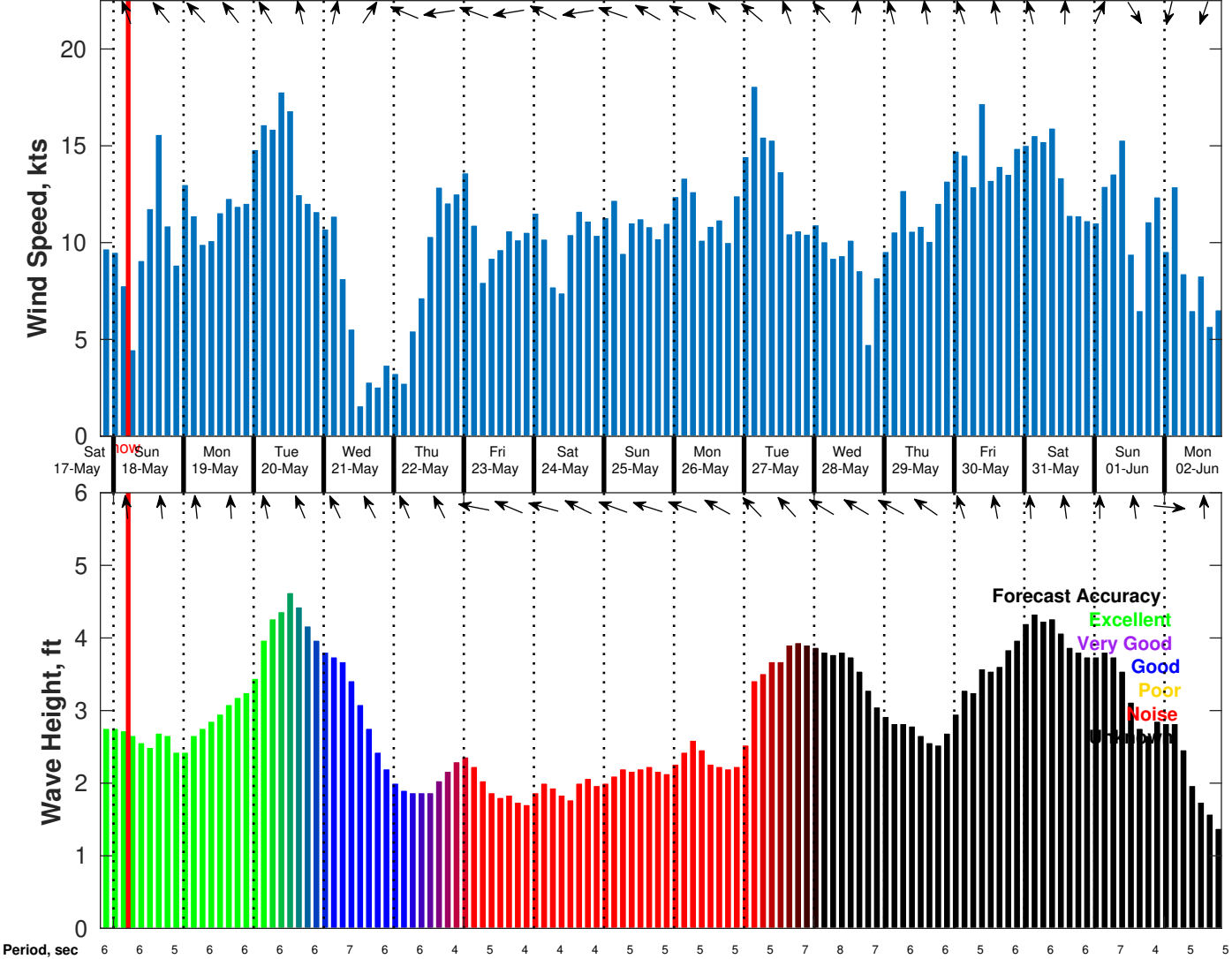
Wind & Wave Forecast for Shell Noches GC19 PPL Geotechnical from 17-May-2025 20:00:00 to 02-Jun-2025 20:00:00
