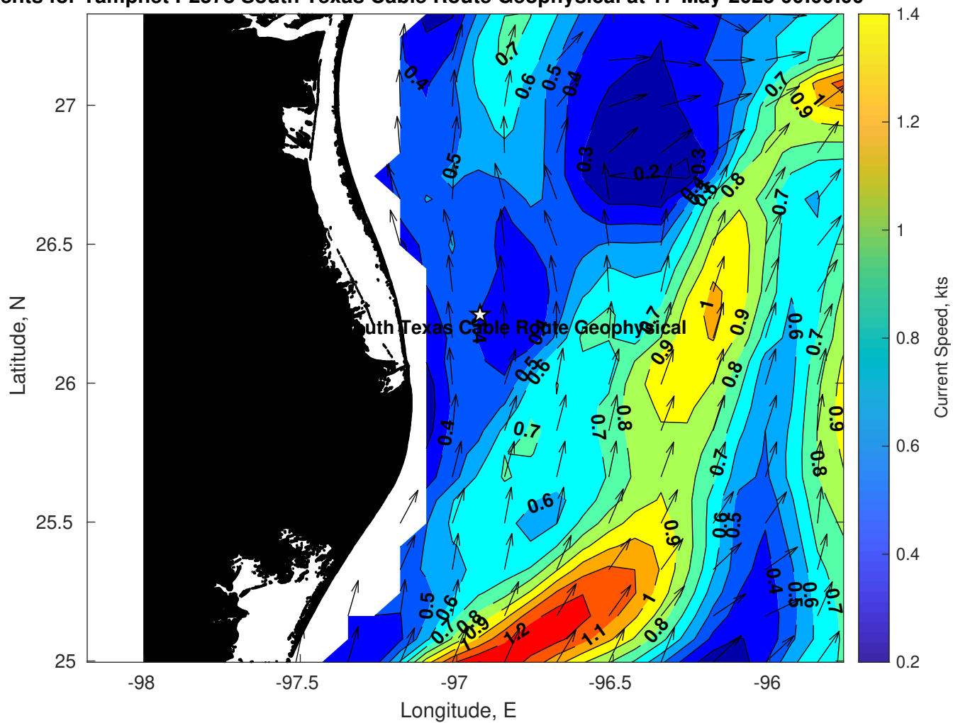
Surface Currents for Tampnet P2378 South Texas Cable Route Geophysical at 17-May-2025 00:00:00
