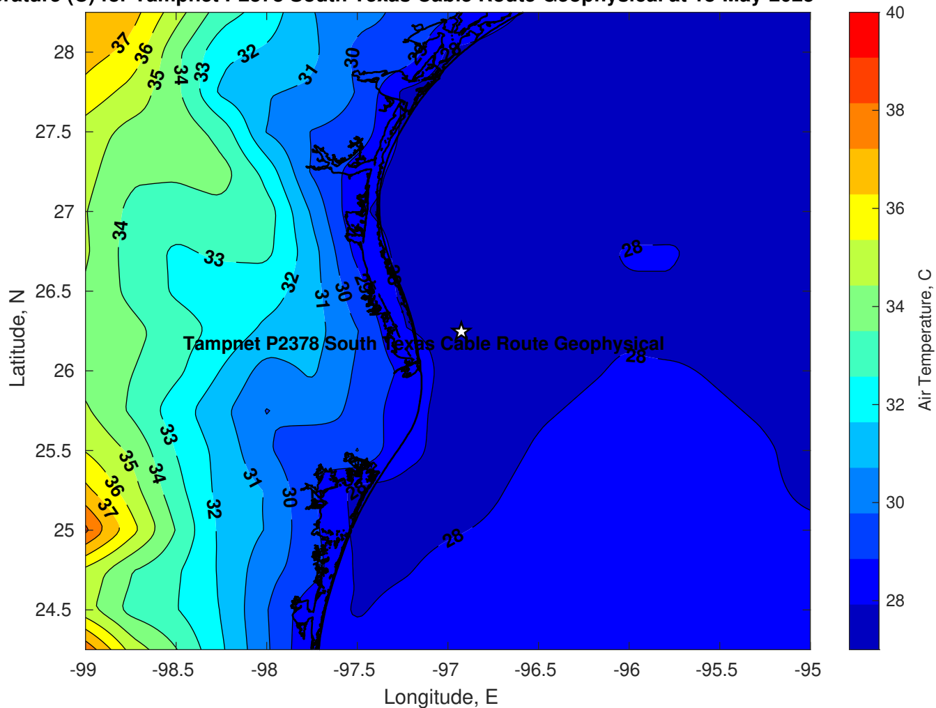
Air Temperature (C) for Tampnet P2378 South Texas Cable Route Geophysical at 18-May-2025
