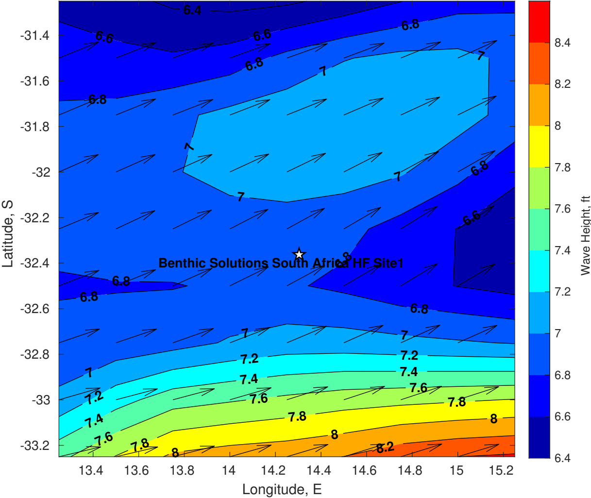
Wave Height (ft) for Benthic Solutions South Africa HF Site1 at 19-May-2025 09:00:00
