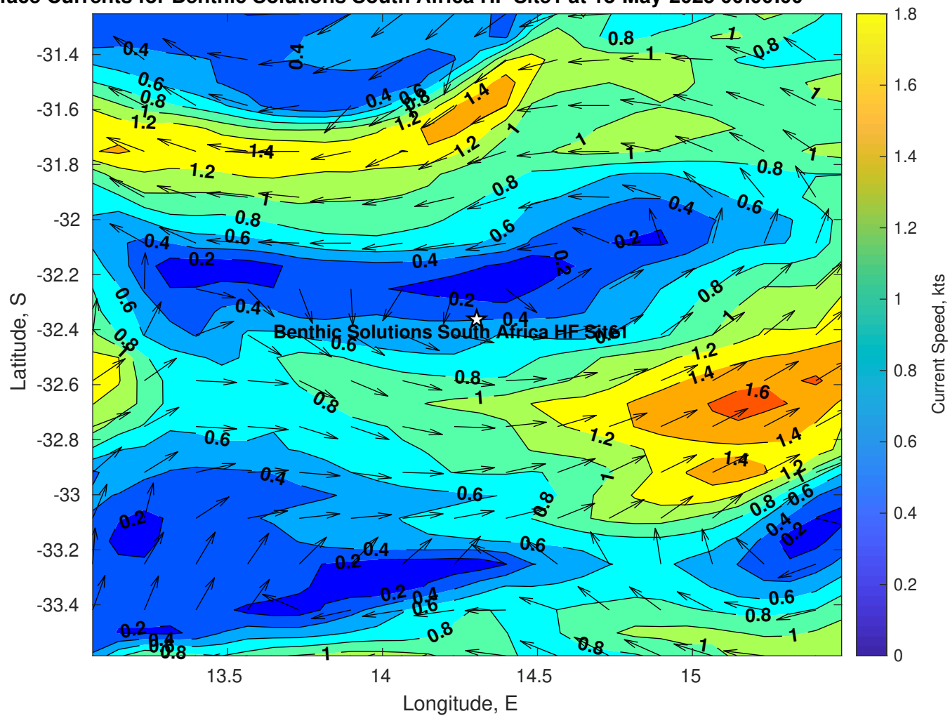
Surface Currents for Benthic Solutions South Africa HF Site1 at 18-May-2025 00:00:00
