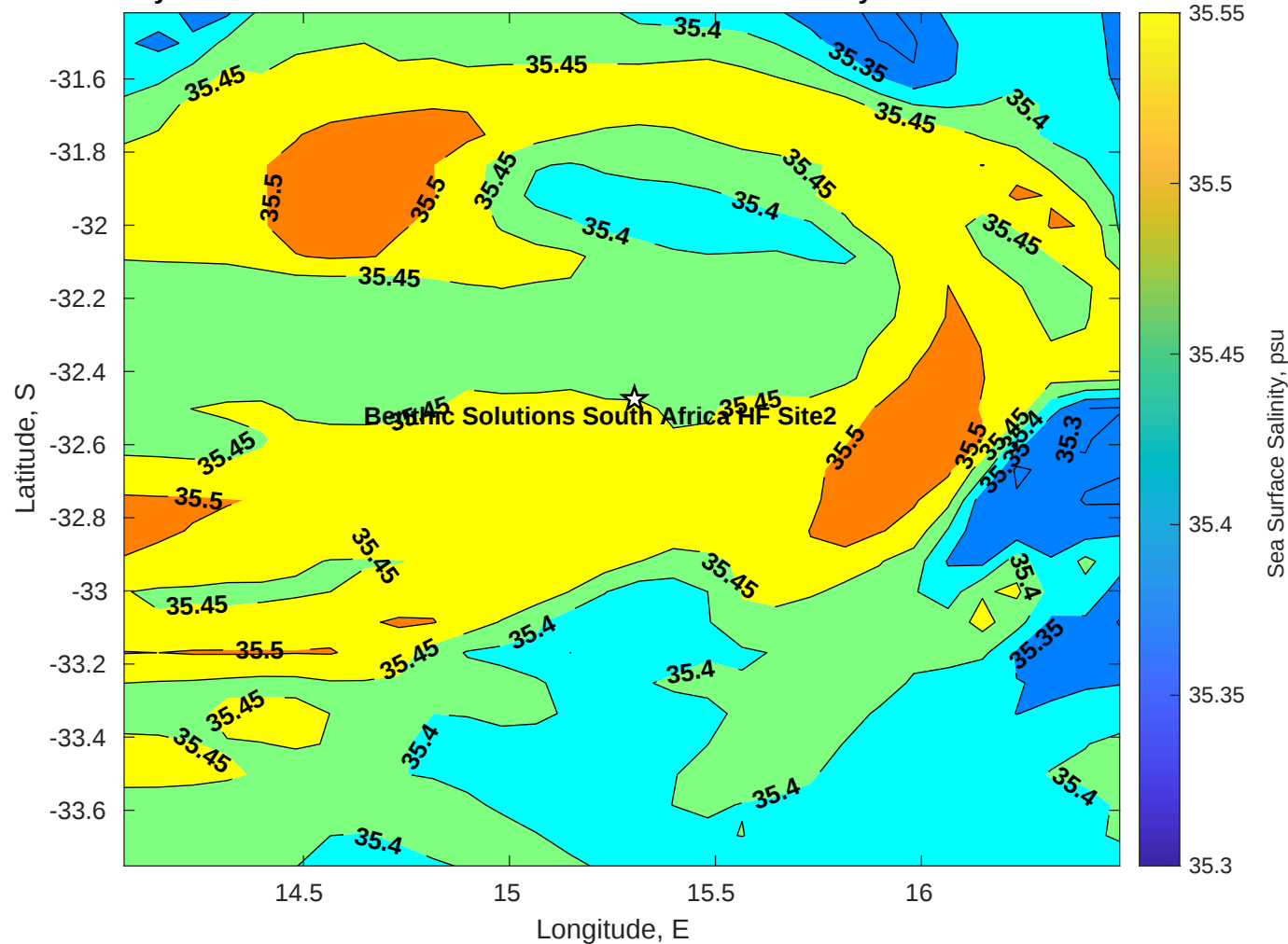
Surface Salinity for Benthic Solutions South Africa HF Site2 at 18-May-2025 00:00:00
