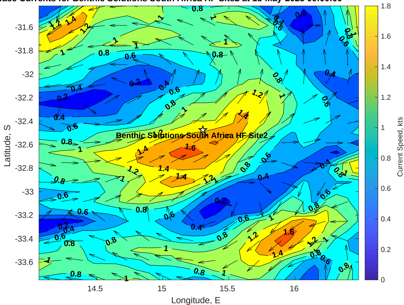
Surface Currents for Benthic Solutions South Africa HF Site2 at 18-May-2025 00:00:00
