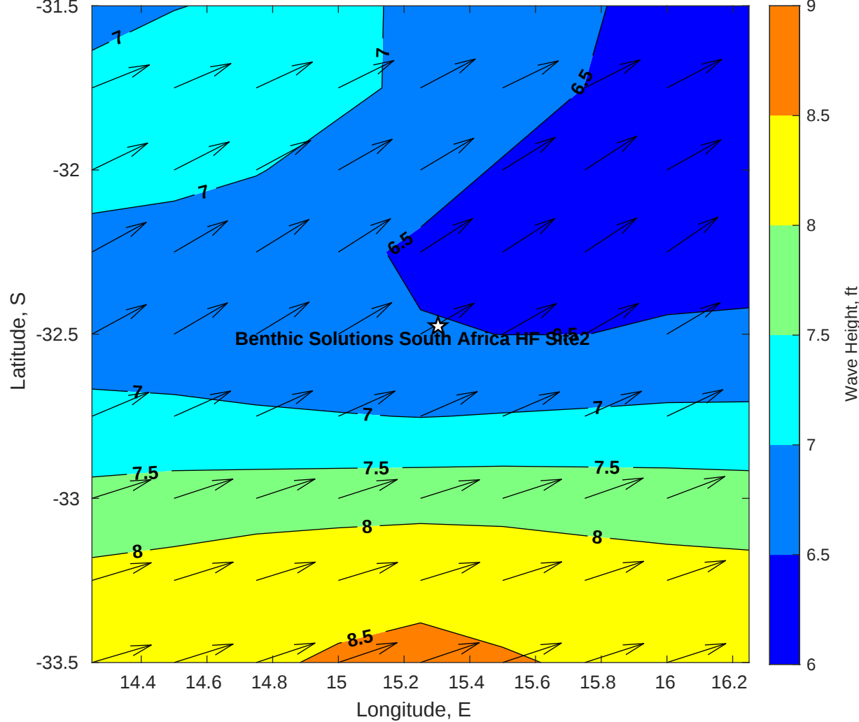
Wave Height (ft) for Benthic Solutions South Africa HF Site2 at 19-May-2025 09:00:00
