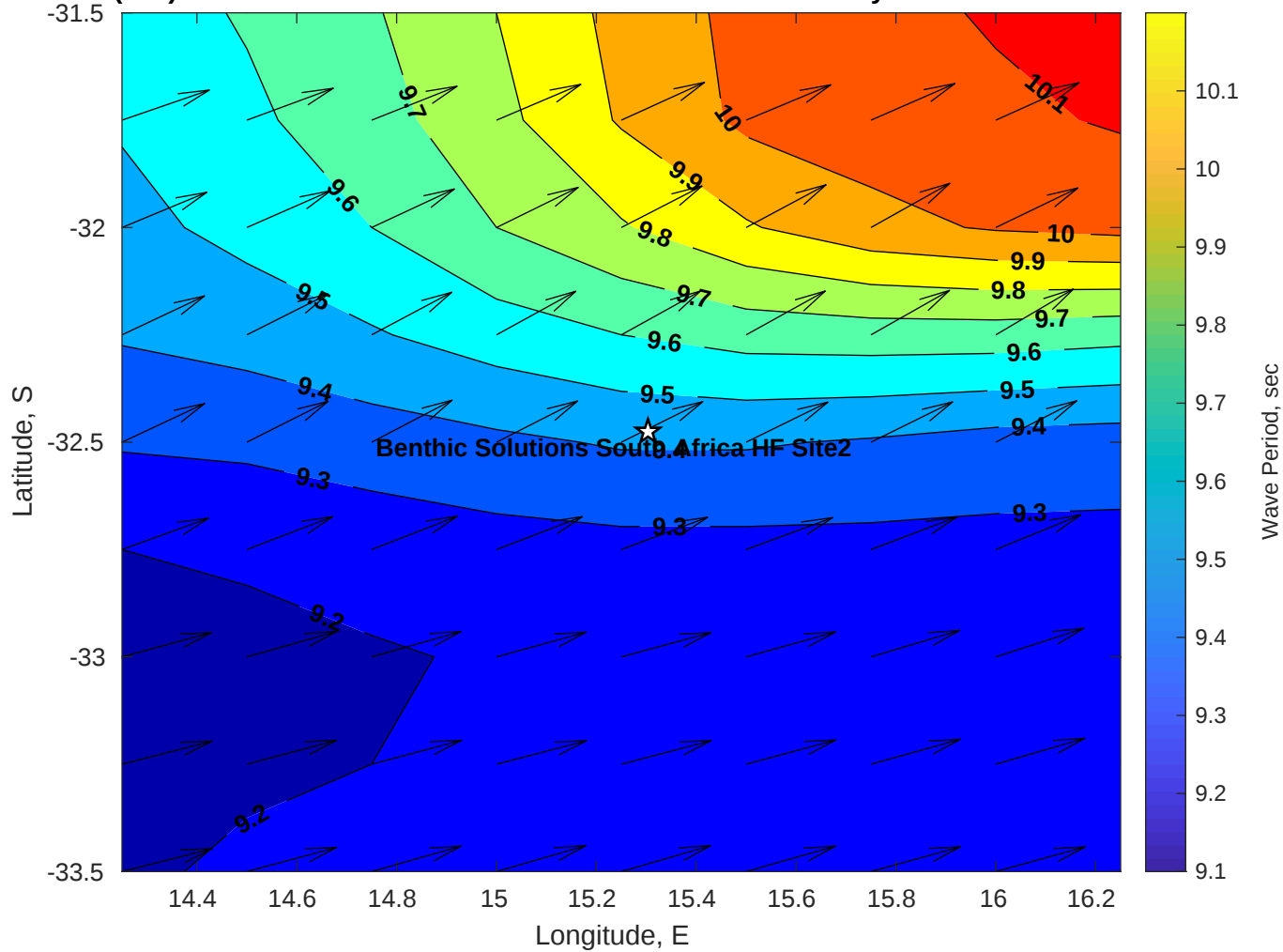
Wave Period (sec) for Benthic Solutions South Africa HF Site2 at 19-May-2025 09:00:00
