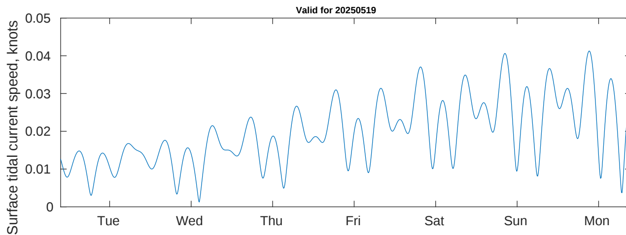
Tidal Currents and Heights for Benthic Solutions South Africa HF Site2 at 20250519
