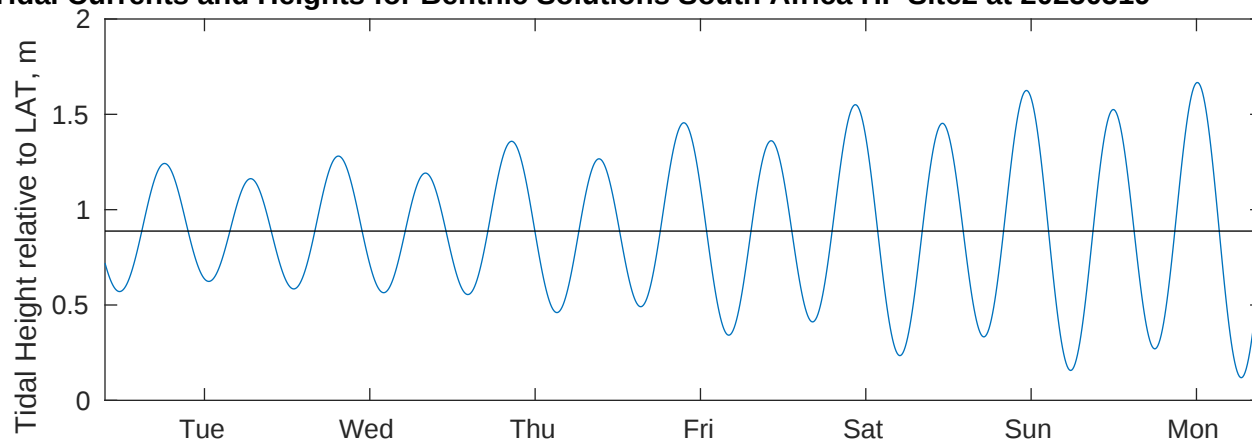
Tidal Currents and Heights for Benthic Solutions South Africa HF Site2 at 20250519
