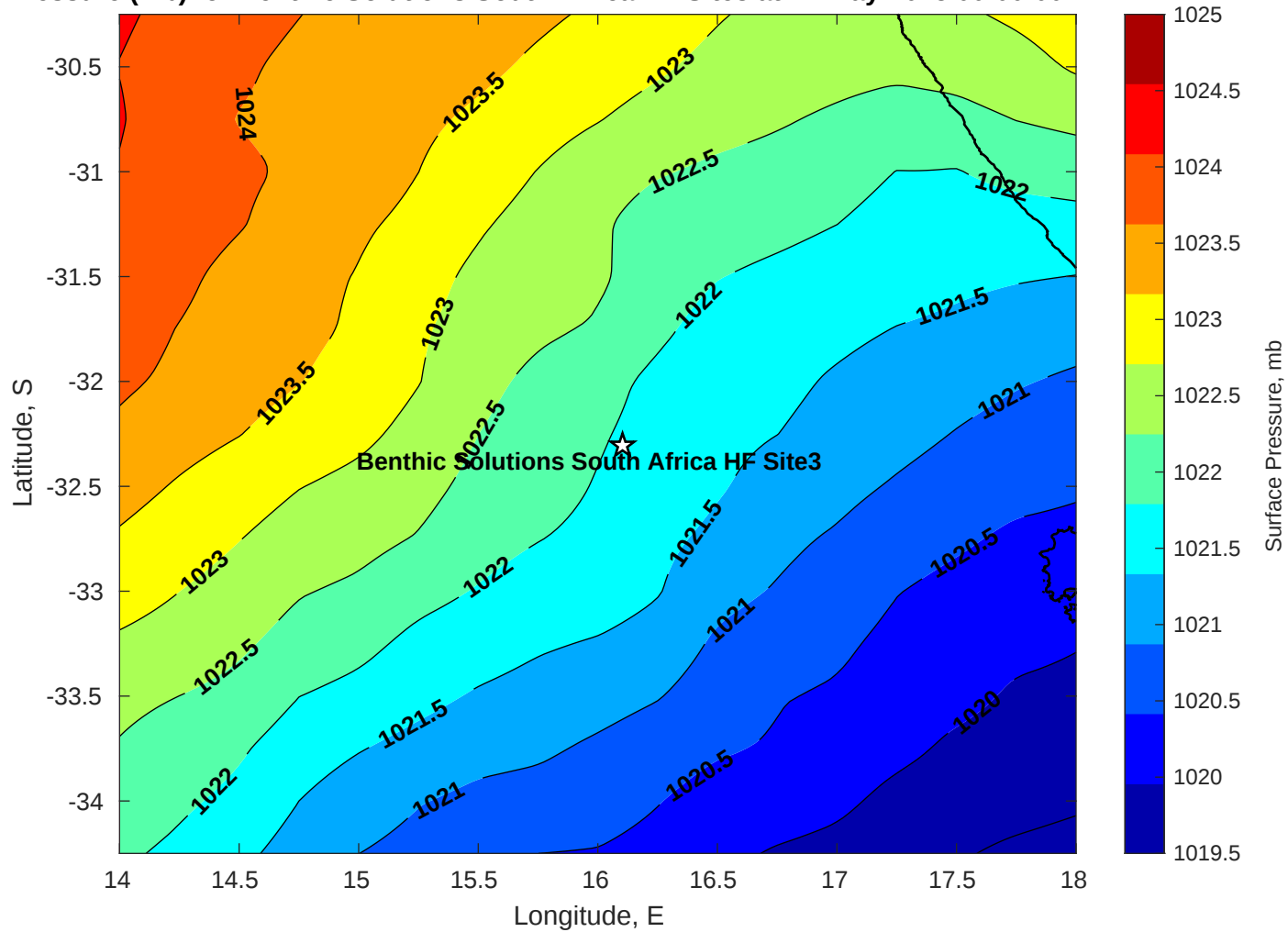
Surface Pressure (mb) for Benthic Solutions South Africa HF Site3 at 21-May-2025 00:00:00
