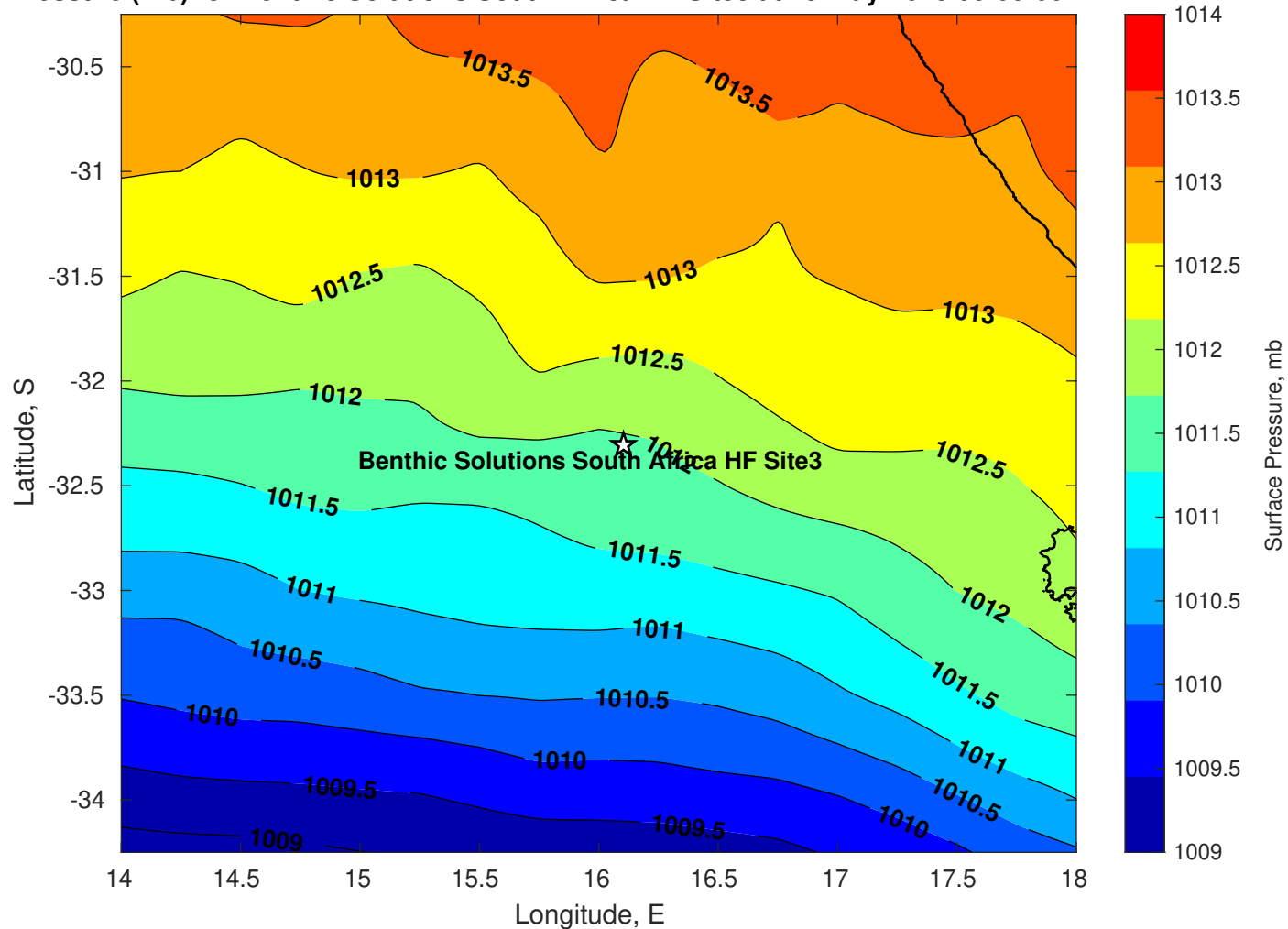
Surface Pressure (mb) for Benthic Solutions South Africa HF Site3 at 19-May-2025 00:00:00
