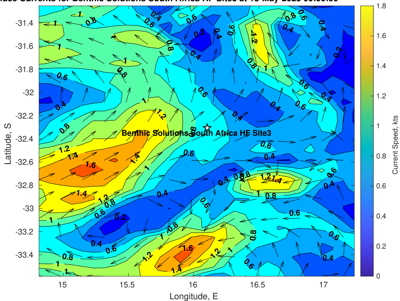
Surface Currents for Benthic Solutions South Africa HF Site3 at 18-May-2025 00:00:00
