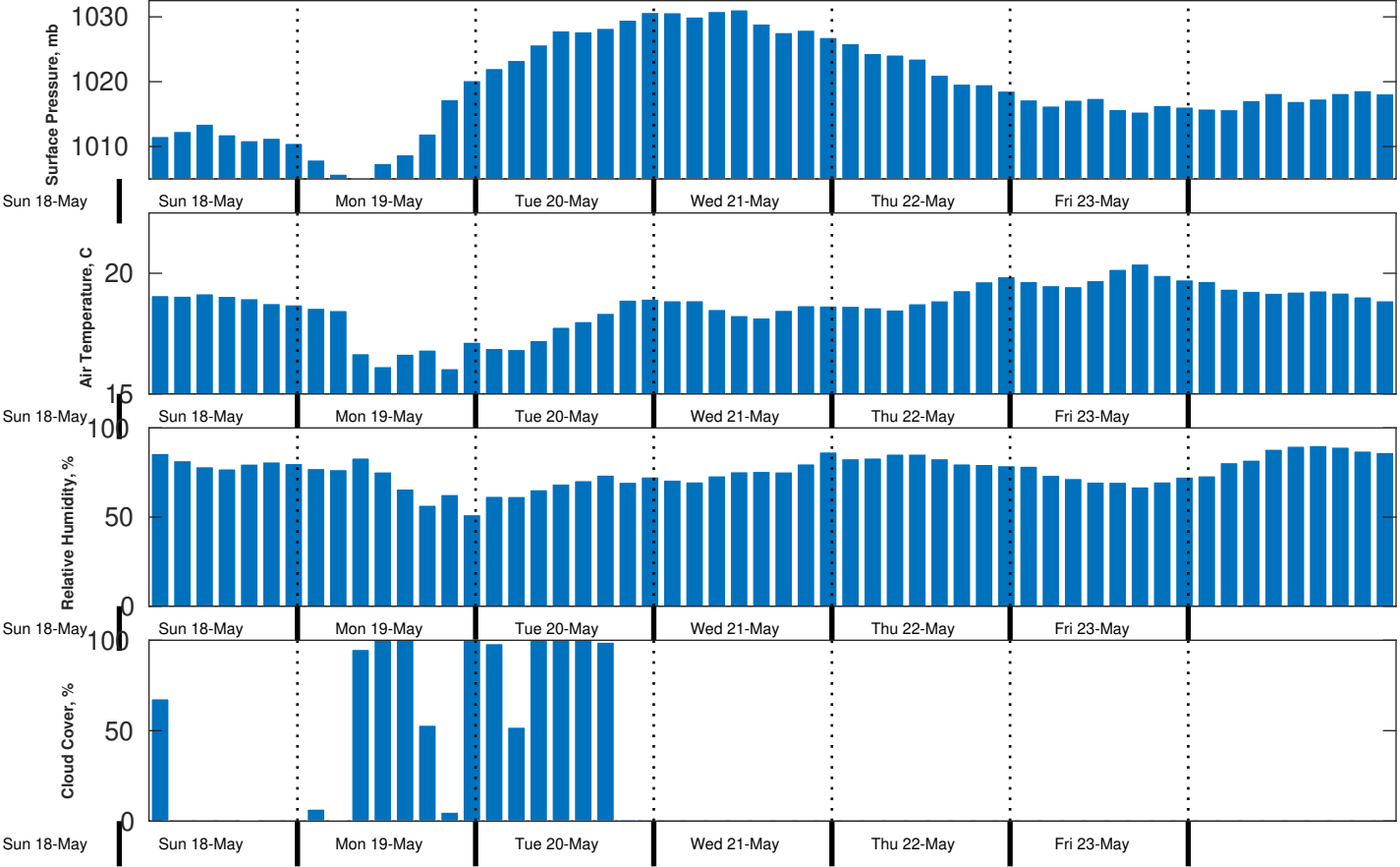
Met Forecast for Benthic Solutions South Africa HF Site3 from 19-May-2025 00:00:00 to 26-May-2025 00:00:00
