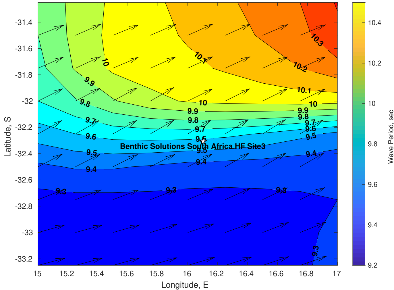
Wave Period (sec) for Benthic Solutions South Africa HF Site3 at 19-May-2025 09:00:00
