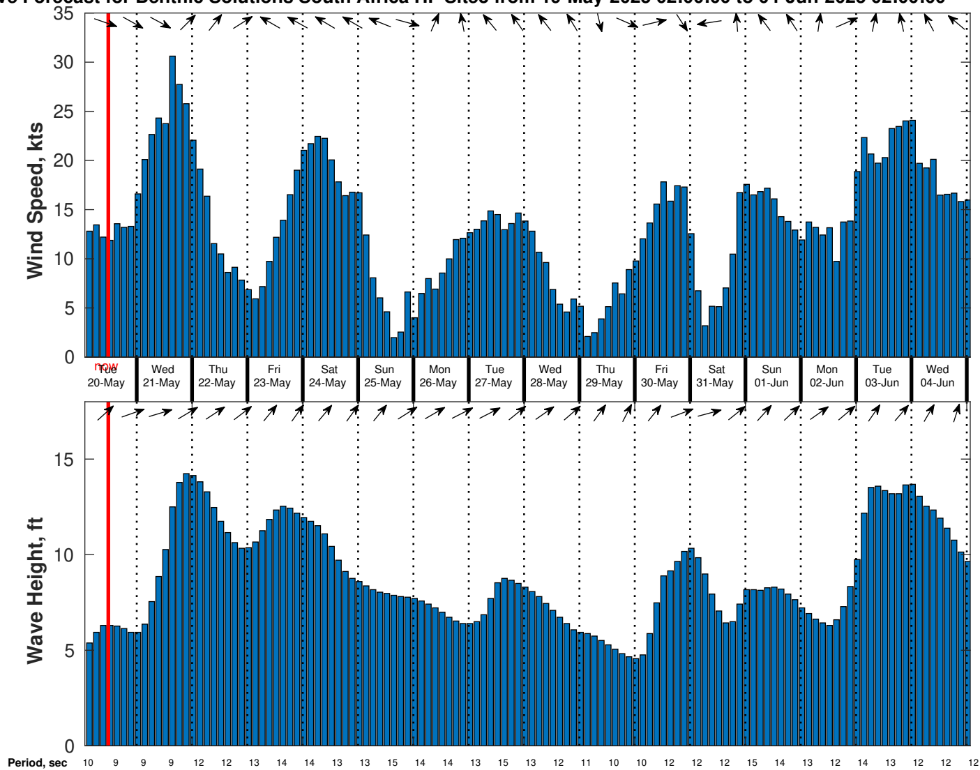
Wind & Wave Forecast for Benthic Solutions South Africa HF Site3 from 19-May-2025 02:00:00 to 04-Jun-2025 02:00:00
