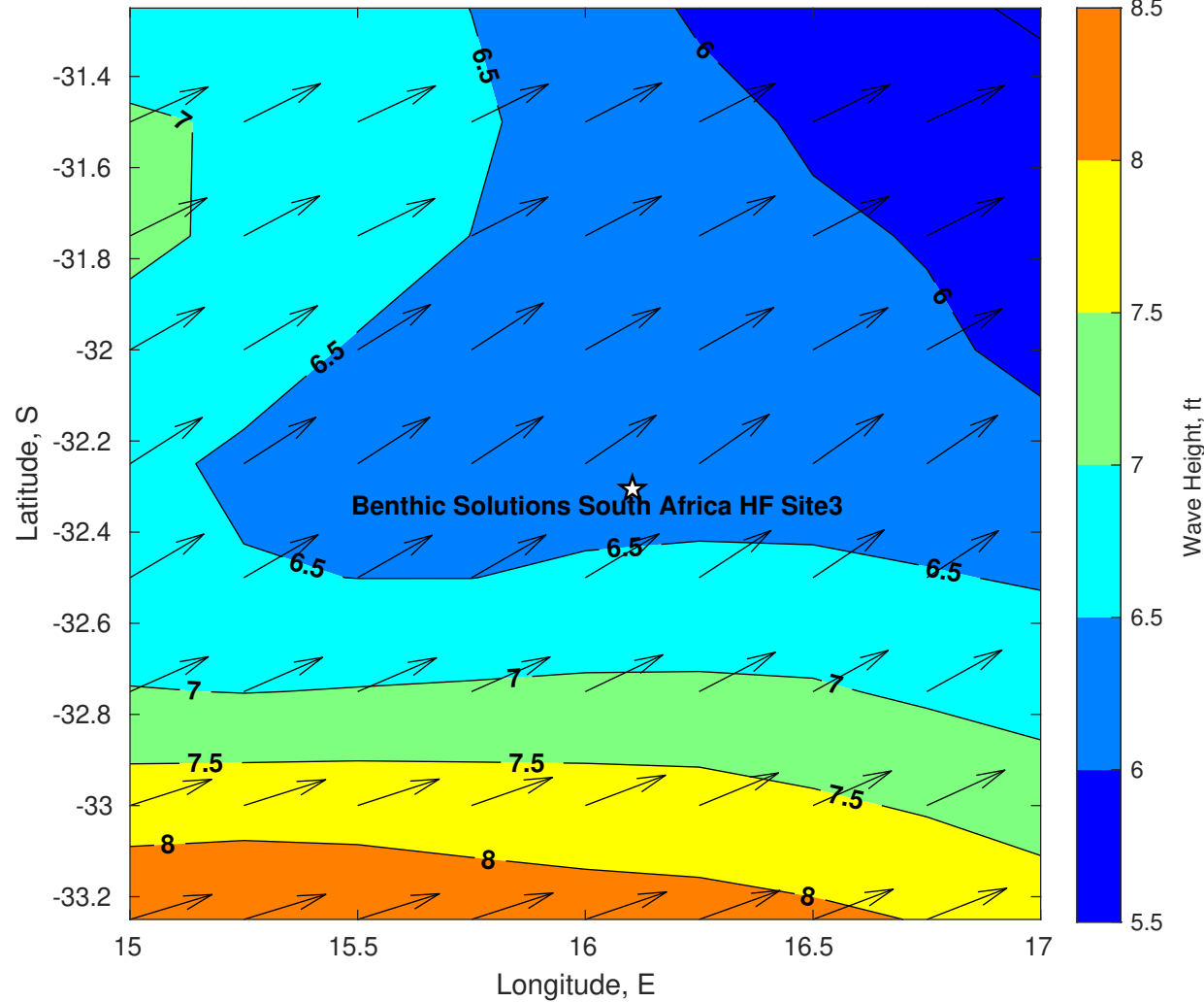
Wave Height (ft) for Benthic Solutions South Africa HF Site3 at 19-May-2025 09:00:00
