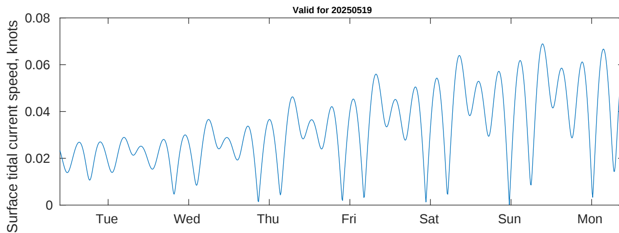
Tidal Currents and Heights for Benthic Solutions South Africa HF Site3 at 20250519
