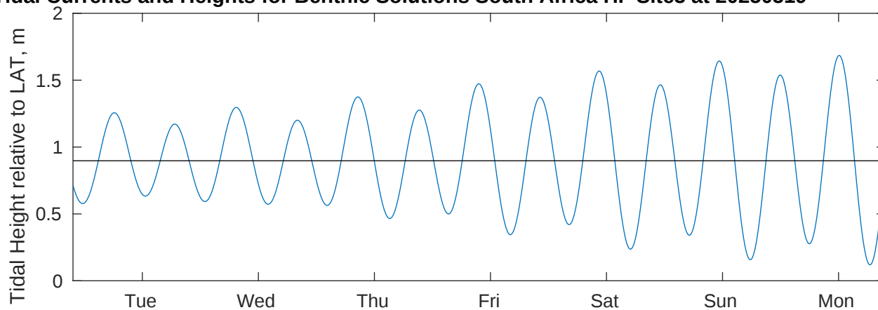
Tidal Currents and Heights for Benthic Solutions South Africa HF Site3 at 20250519
