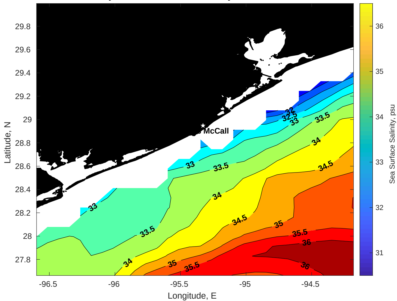
Surface Salinity for Brooks McCall at 18-May-2025 00:00:00
