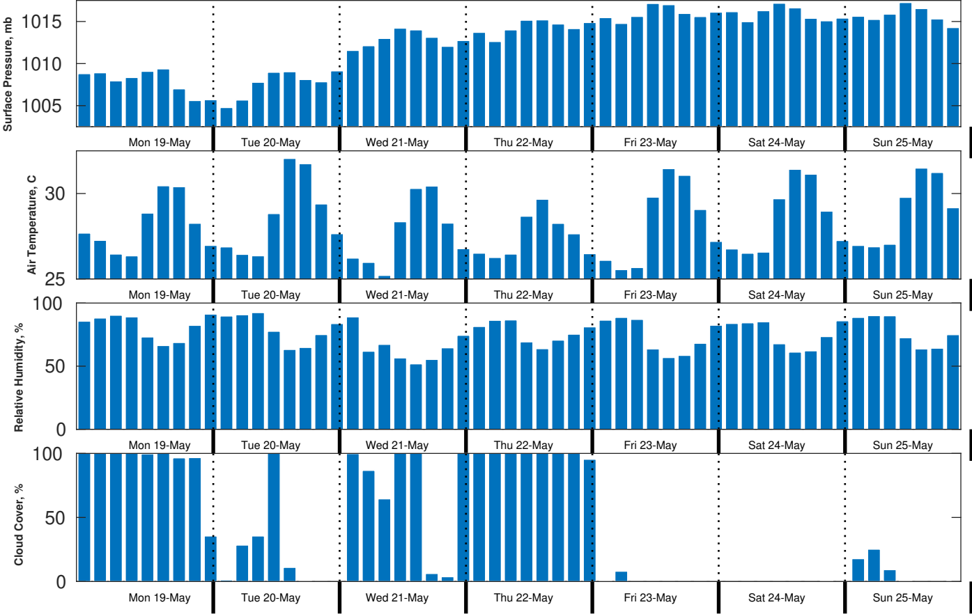
Met Forecast for Brooks McCall from 19-May-2025 00:00:00 to 26-May-2025 00:00:00
