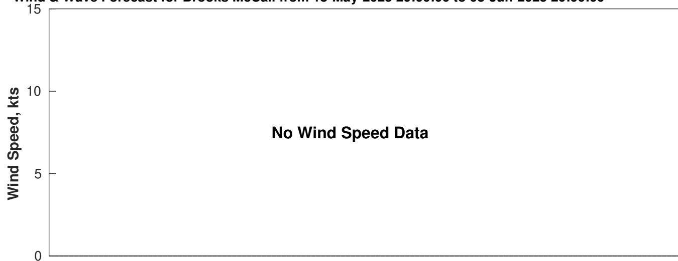
Wind & Wave Forecast for Brooks McCall from 18-May-2025 20:00:00 to 03-Jun-2025 20:00:00
