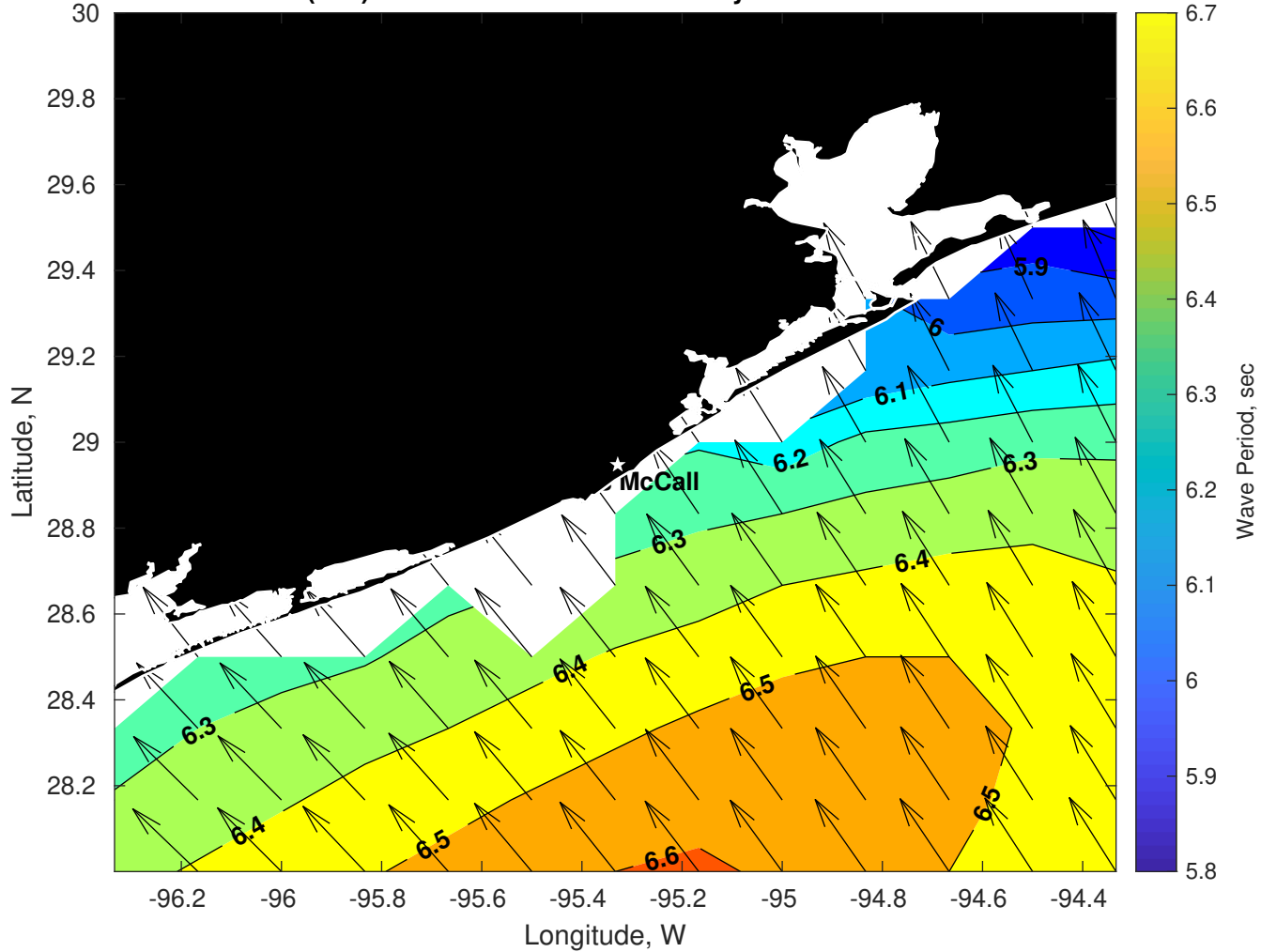
Wave Period (sec) for Brooks McCall at 19-May-2025 09:00:00
