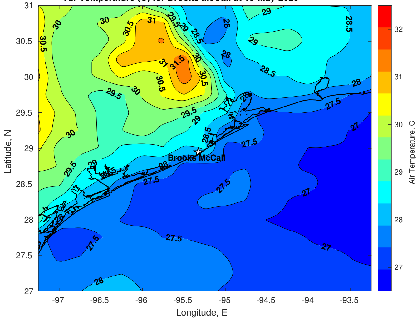
Air Temperature (C) for Brooks McCall at 19-May-2025
