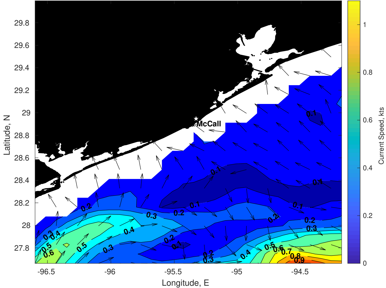
Surface Currents for Brooks McCall at 18-May-2025 00:00:00
