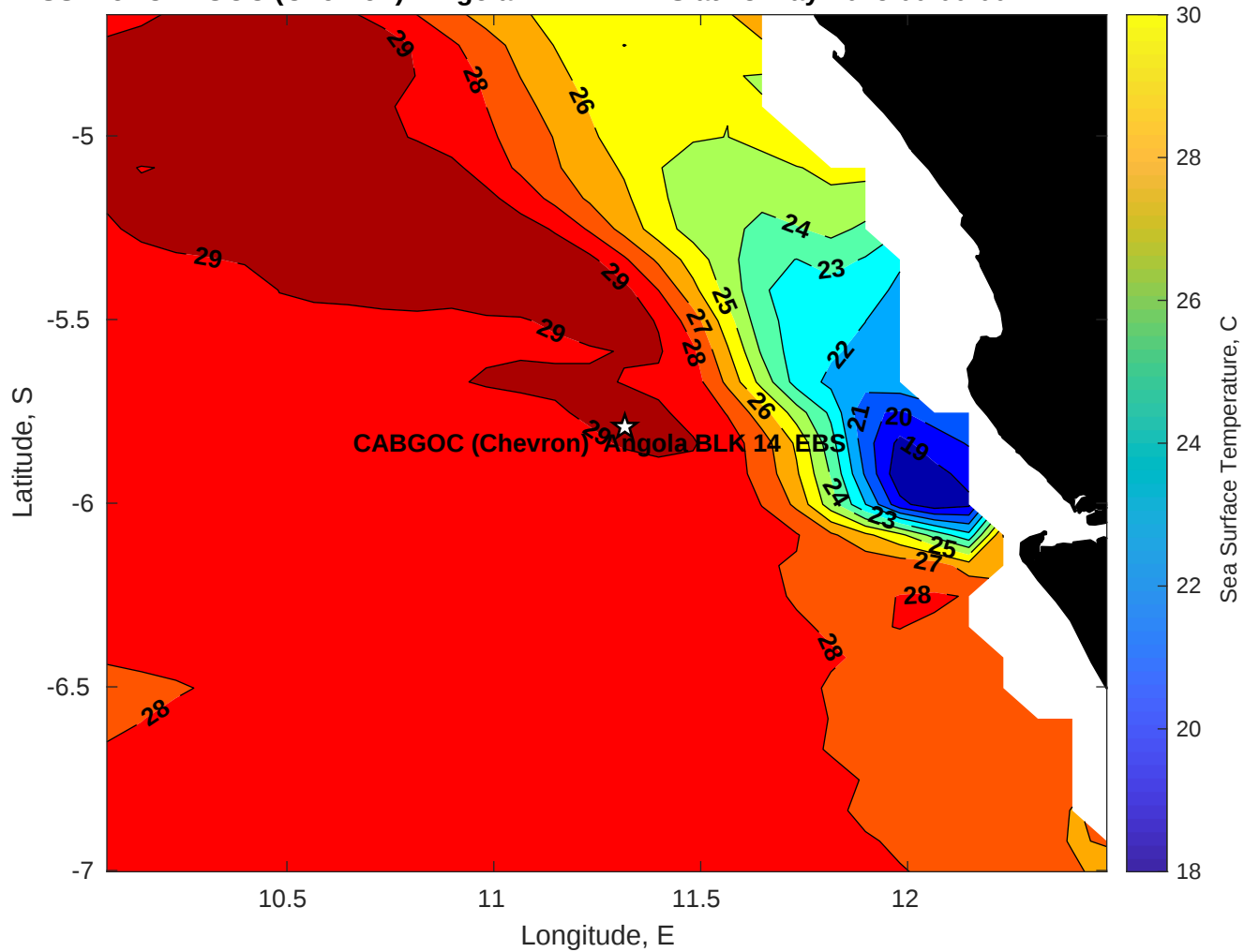
SST for CABGOC (Chevron) Angola BLK 14 EBS at 18-May-2025 00:00:00
