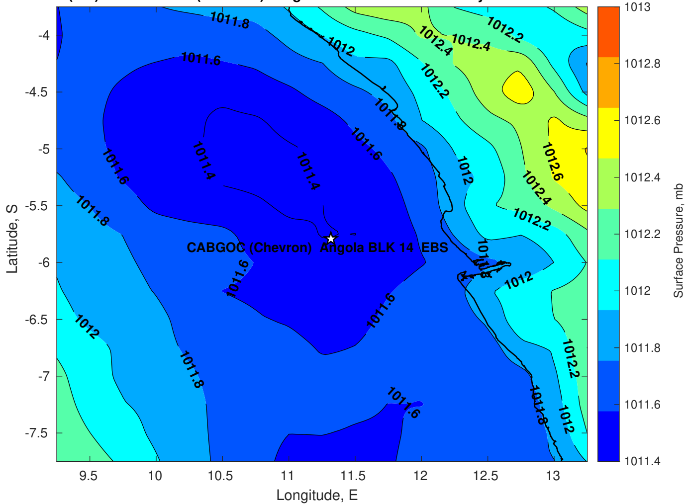
Surface Pressure (mb) for CABGOC (Chevron) Angola BLK 14 EBS at 20-May-2025 00:00:00
