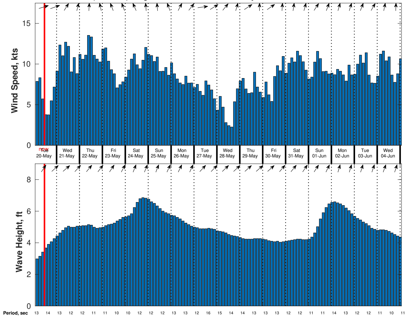
Wind & Wave Forecast for CABGOC (Chevron) Angola BLK 14 EBS from 19-May-2025 02:00:00 to 04-Jun-2025 02:00:00
