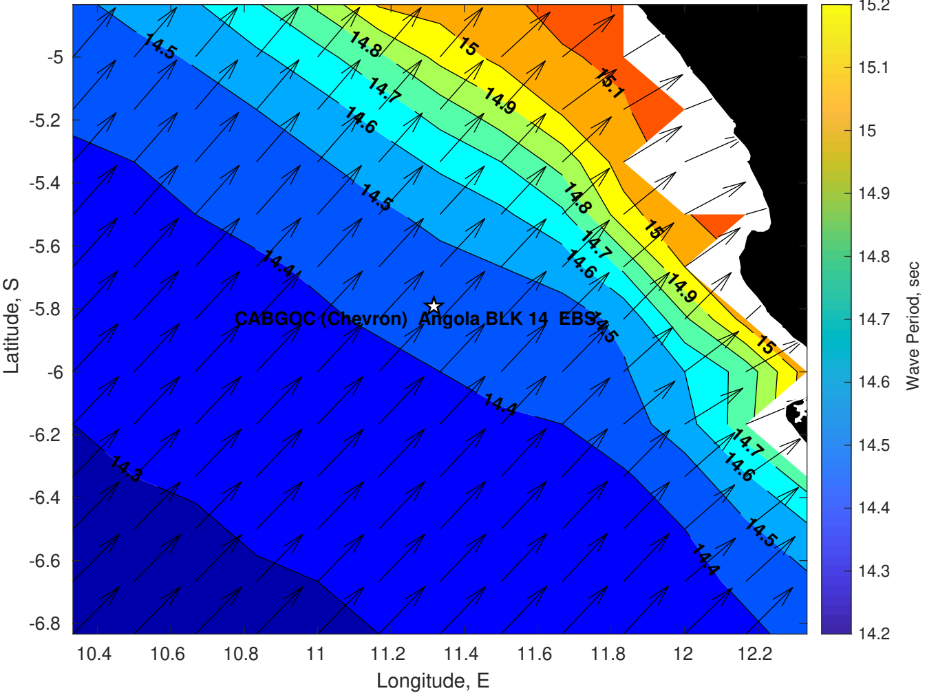
Wave Period (sec) for CABGOC (Chevron) Angola BLK 14 EBS at 19-May-2025 09:00:00
