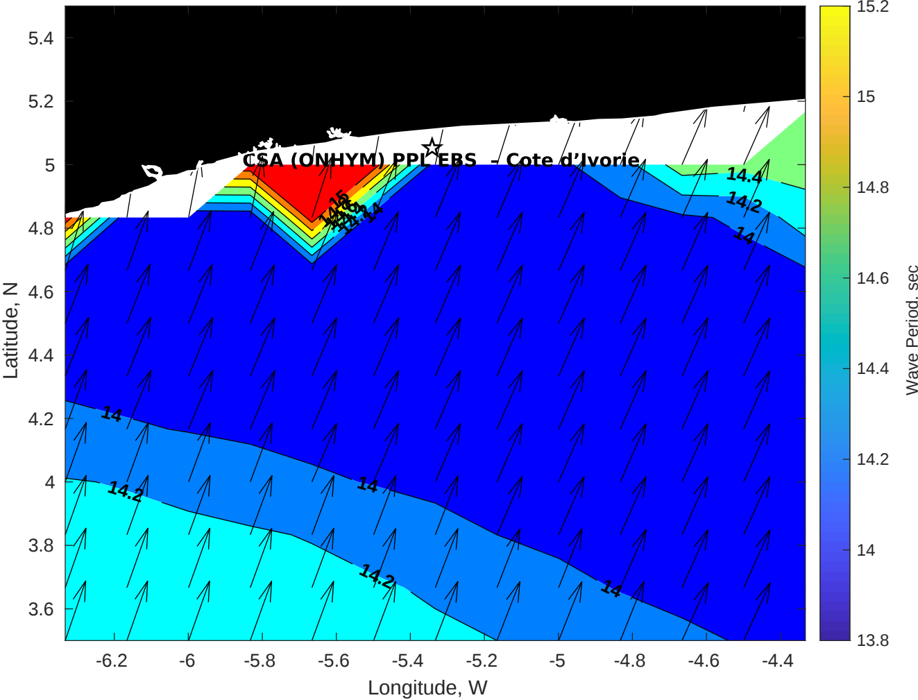
Wave Period (sec) for CSA (ONHYM) PPL EBS - Cote d'Ivoire at 19-May-2025 09:00:00
