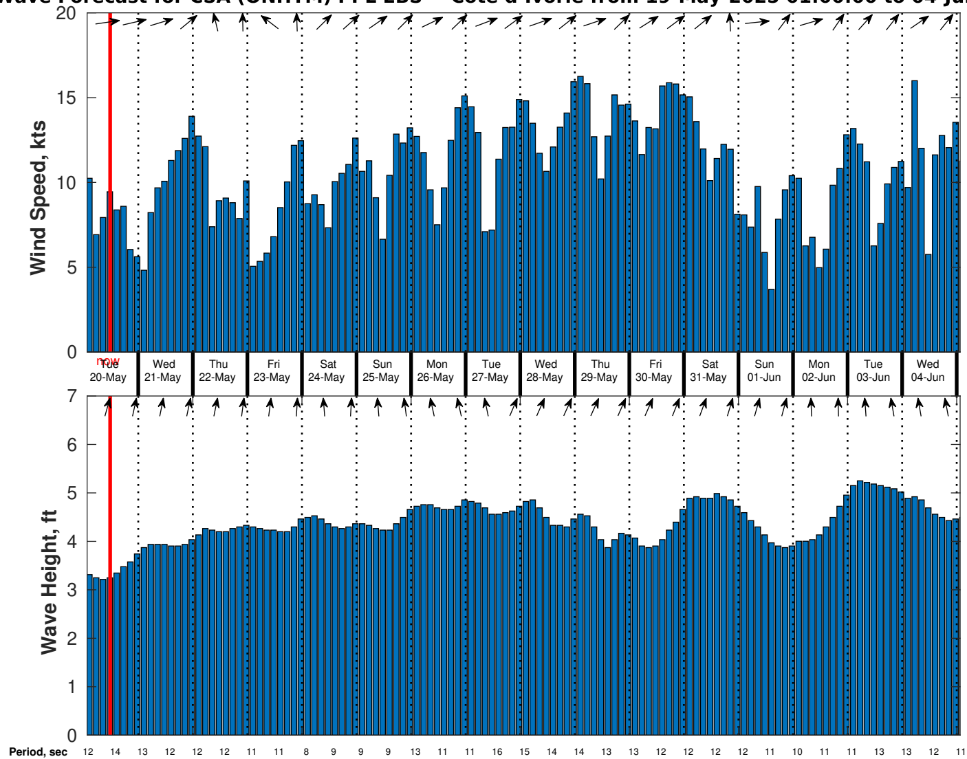
Wind & Wave Forecast for CSA (ONHYM) PPL EBS - Cote d'Ivoire from 19-May-2025 01:00:00 to 04-Jun-2025 01:00:00
