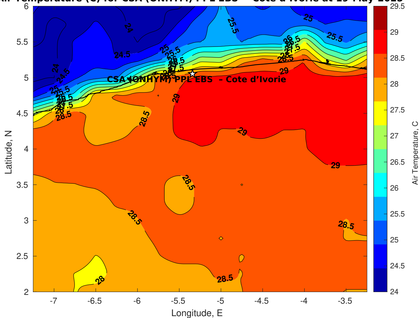
Air Temperature (C) for CSA (ONHYM) PPL EBS - Cote d'Ivoire at 19-May-2025
