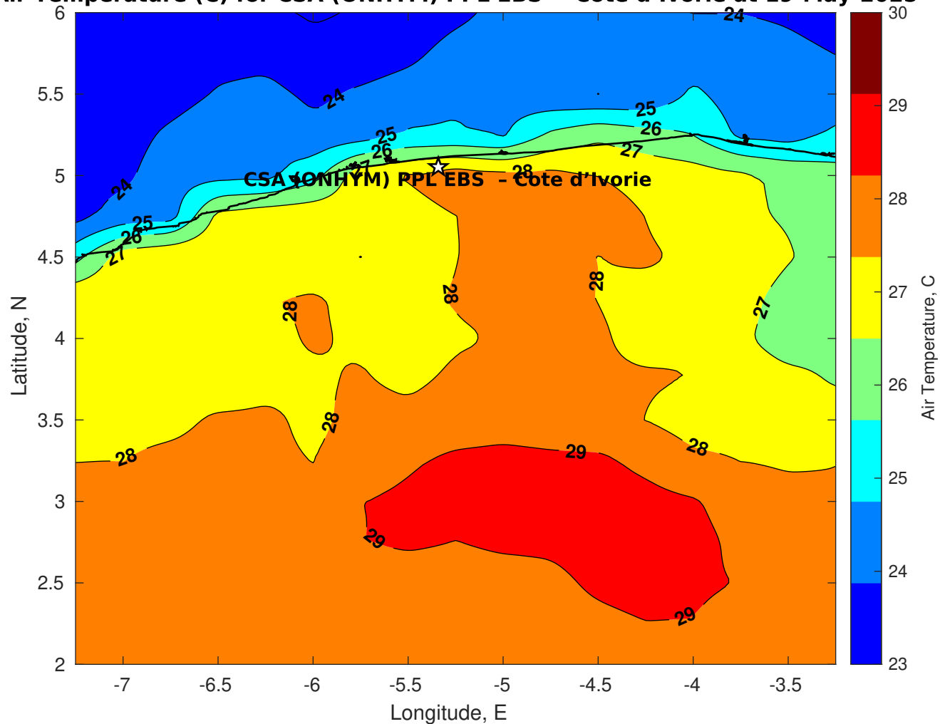
Air Temperature (C) for CSA (ONHYM) PPL EBS - Cote d'Ivoire at 19-May-2025
