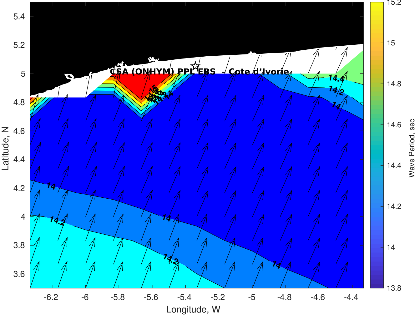
Wave Period (sec) for CSA (ONHYM) PPL EBS - Cote d'Ivoire at 19-May-2025 09:00:00
