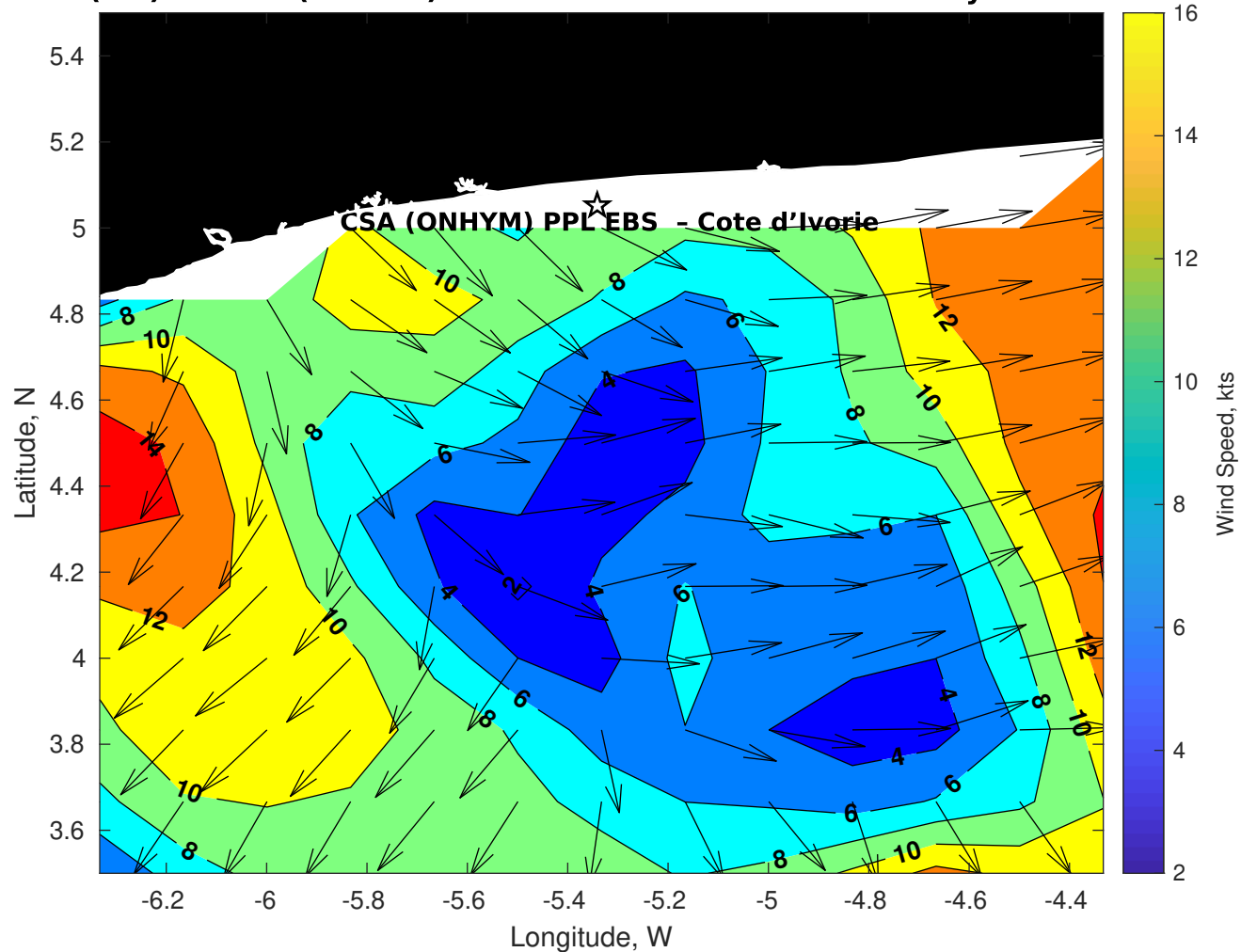
Winds (kts) for CSA (ONHYM) PPL EBS - Cote d'Ivoire at 19-May-2025 09:00:00
