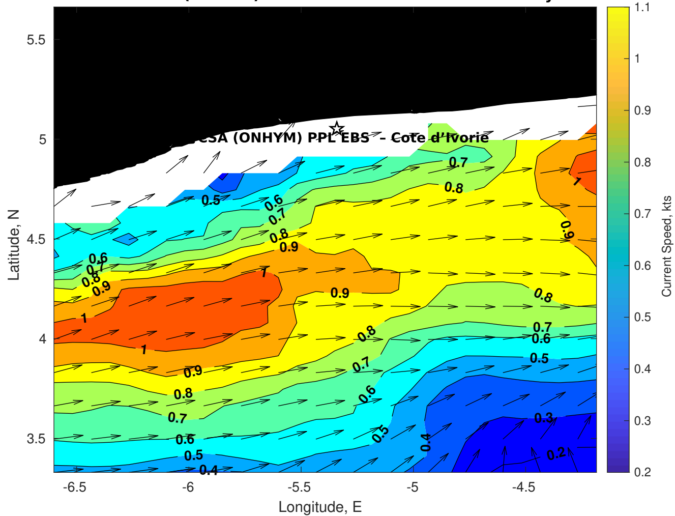
Surface Currents for CSA (ONHYM) PPL EBS - Cote d'Ivoire at 18-May-2025 00:00:00
