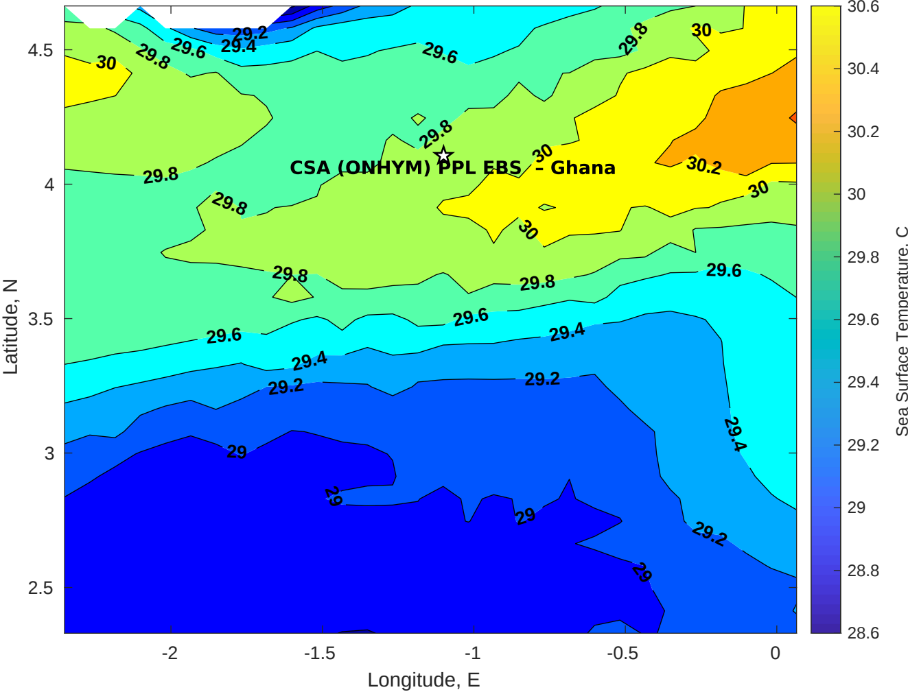
SST for CSA (ONHYM) PPL EBS - Ghana at 18-May-2025 00:00:00
