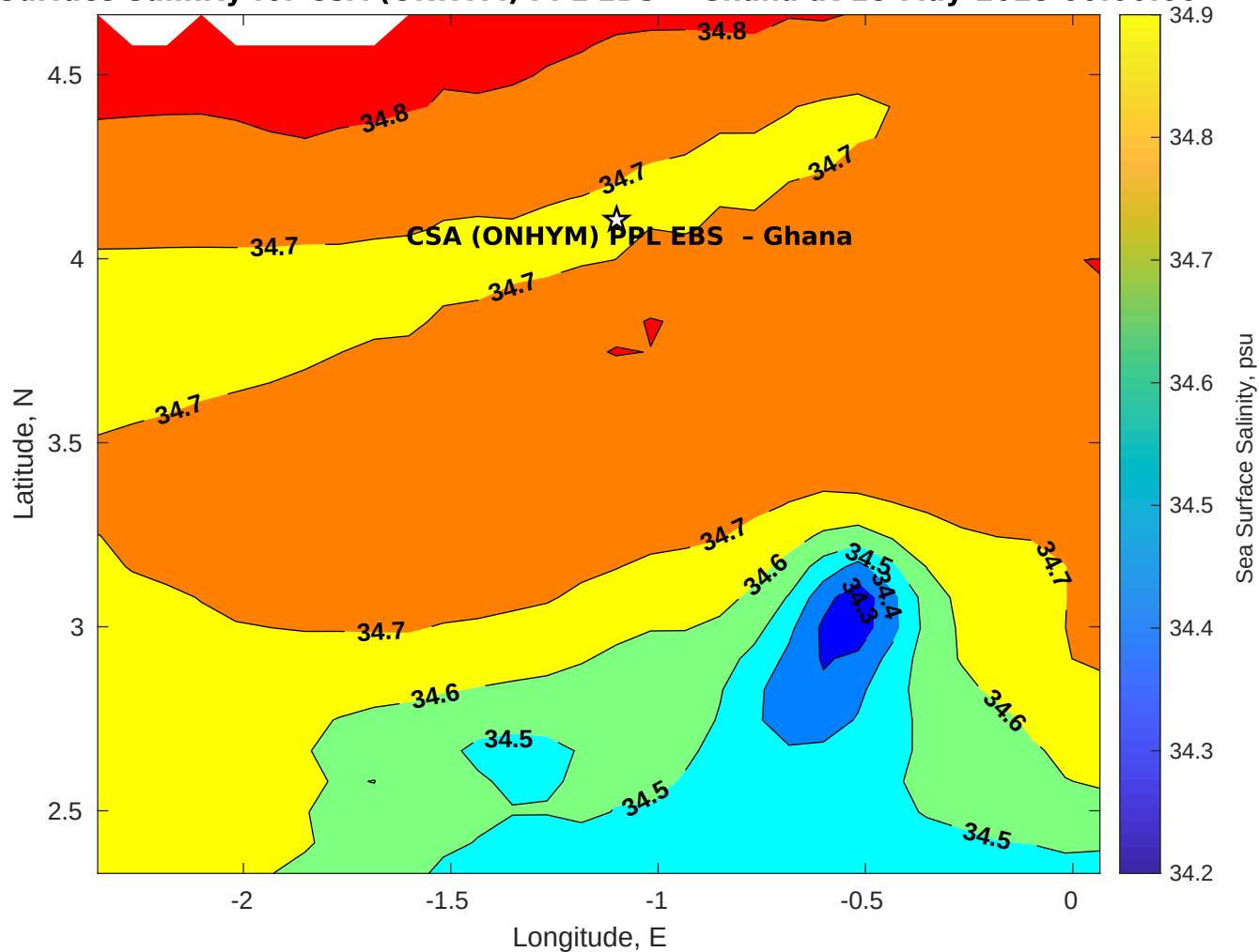
Surface Salinity for CSA (ONHYM) PPL EBS - Ghana at 18-May-2025 00:00:00
