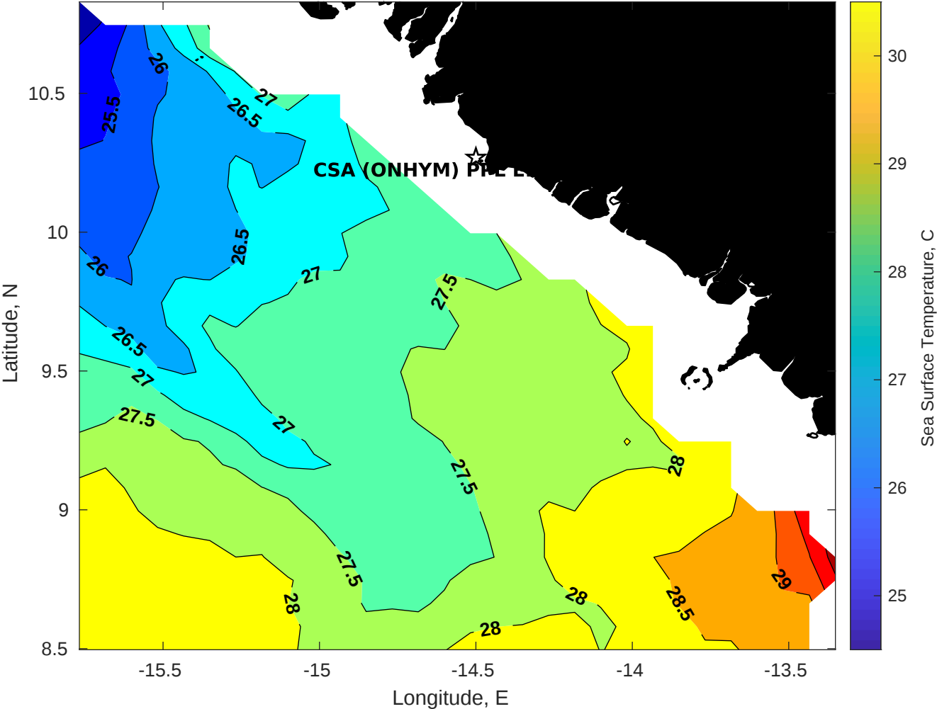
SST for CSA (ONHYM) PPL EBS - Guinea at 18-May-2025 00:00:00
