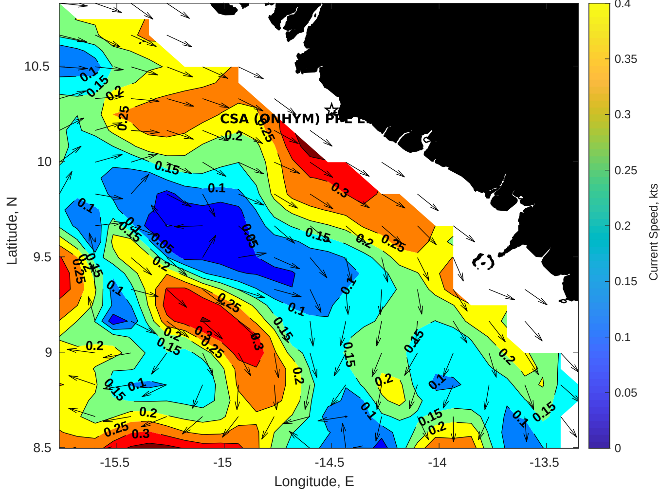
Surface Currents for CSA (ONHYM) PPL EBS - Guinea at 18-May-2025 00:00:00
