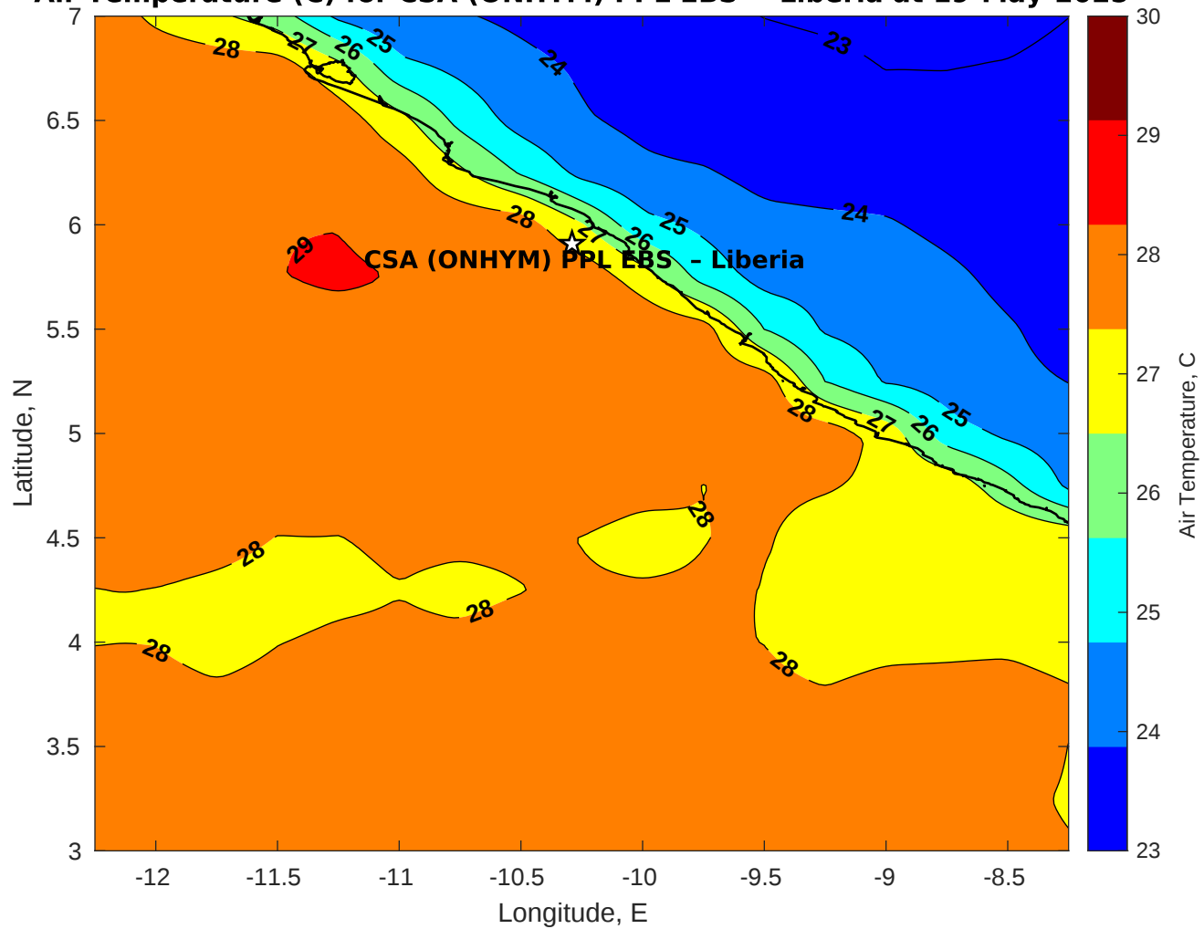
Air Temperature (C) for CSA (ONHYM) PPL EBS - Liberia at 19-May-2025
