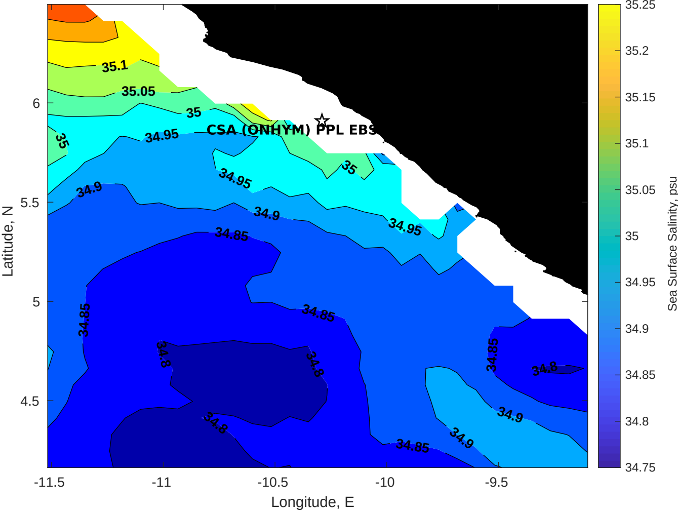
Surface Salinity for CSA (ONHYM) PPL EBS - Liberia at 18-May-2025 00:00:00
