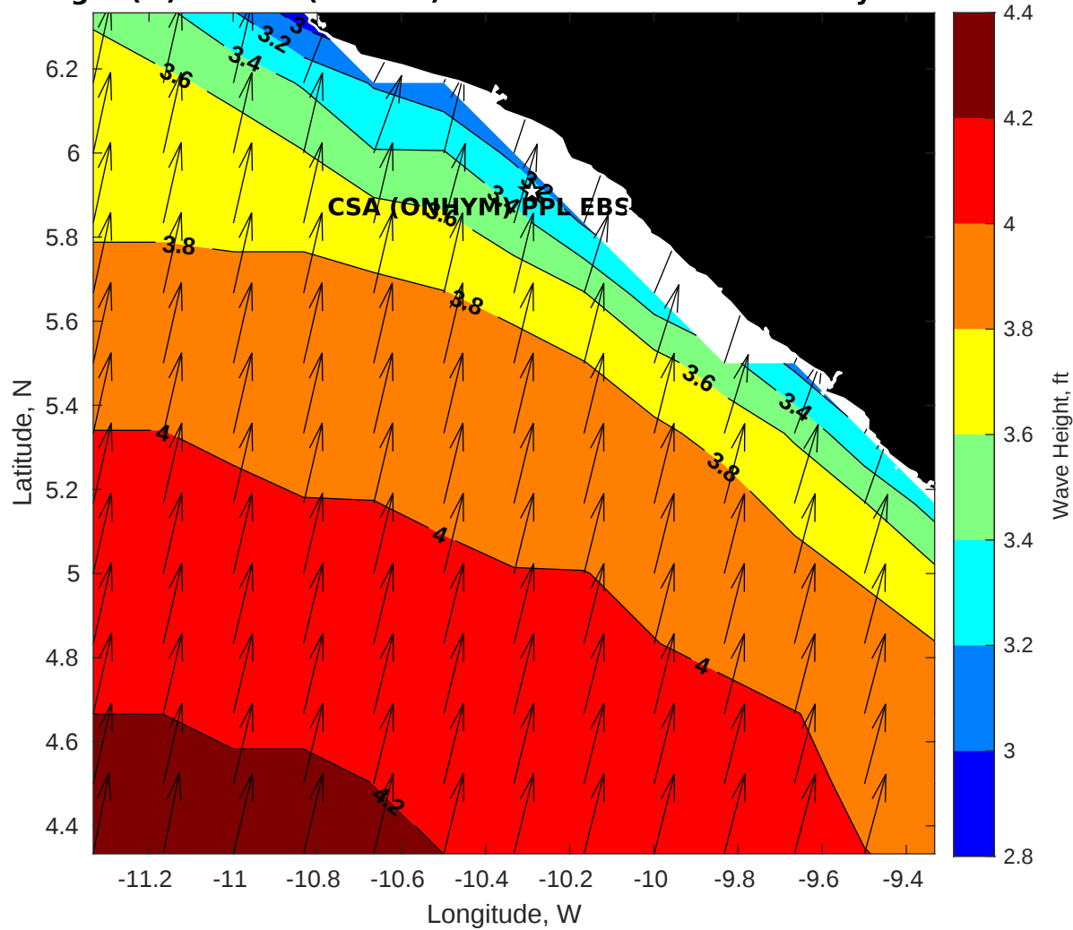
Wave Height (ft) for CSA (ONHYM) PPL EBS - Liberia at 19-May-2025 09:00:00
