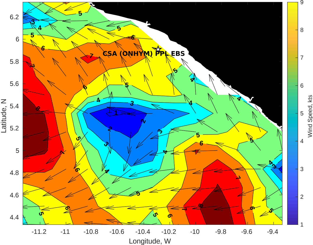
Winds (kts) for CSA (ONHYM) PPL EBS - Liberia at 19-May-2025 09:00:00
