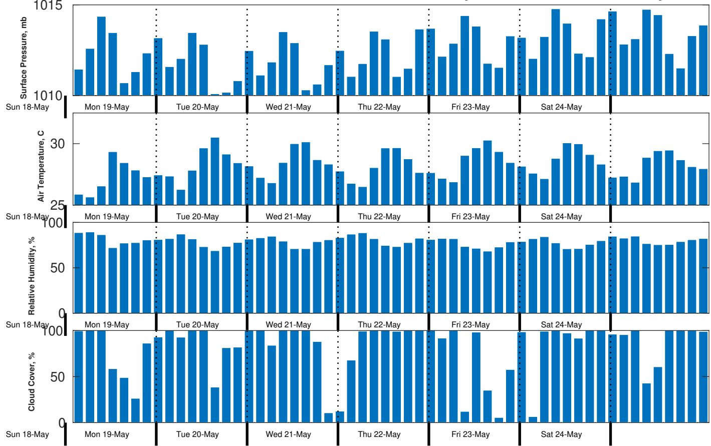
Met Forecast for CSA (ONHYM) PPL EBS - Liberia from 19-May-2025 00:00:00 to 26-May-2025 00:00:00
