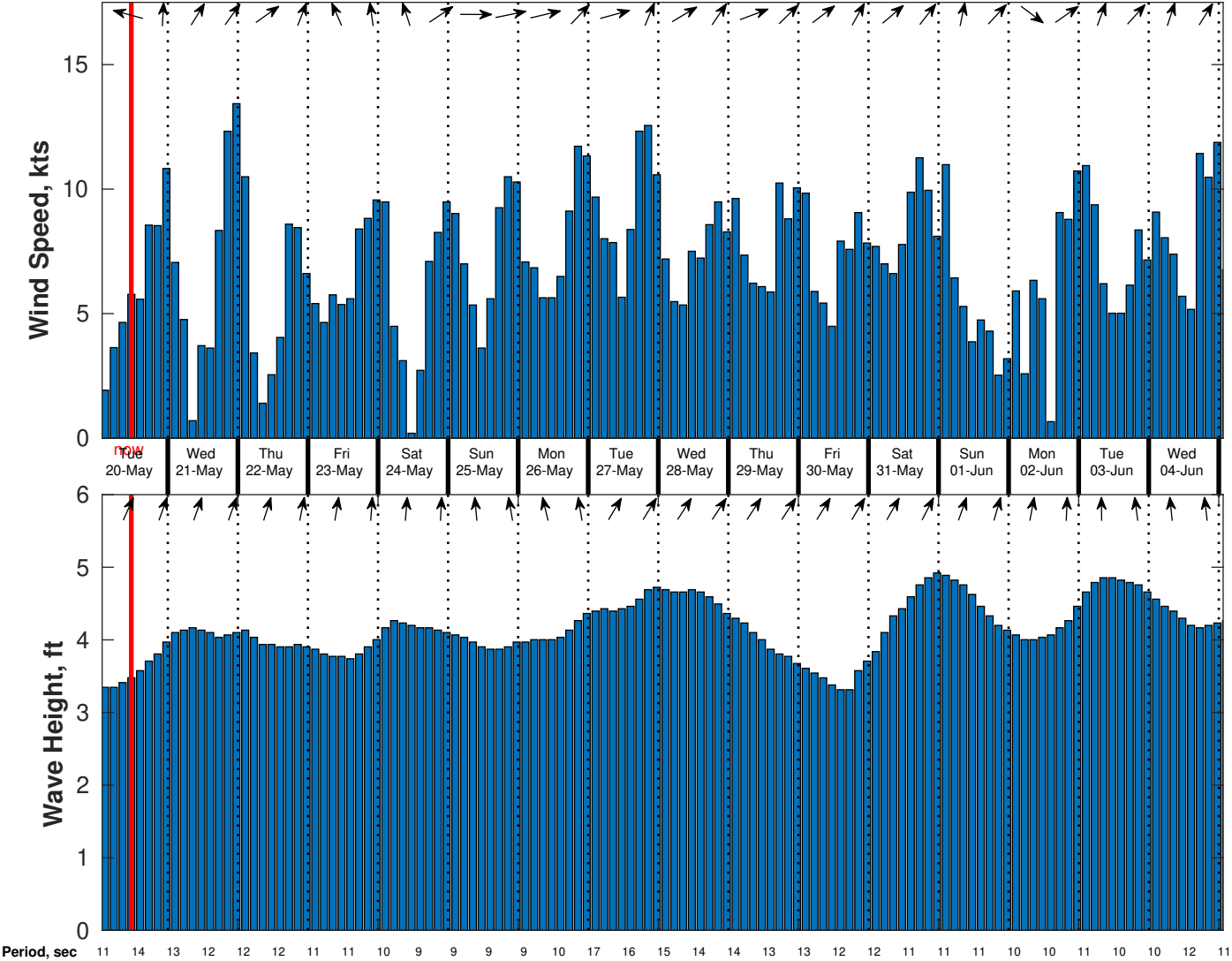
Wind & Wave Forecast for CSA (ONHYM) PPL EBS - Liberia from 19-May-2025 01:00:00 to 04-Jun-2025 01:00:00
