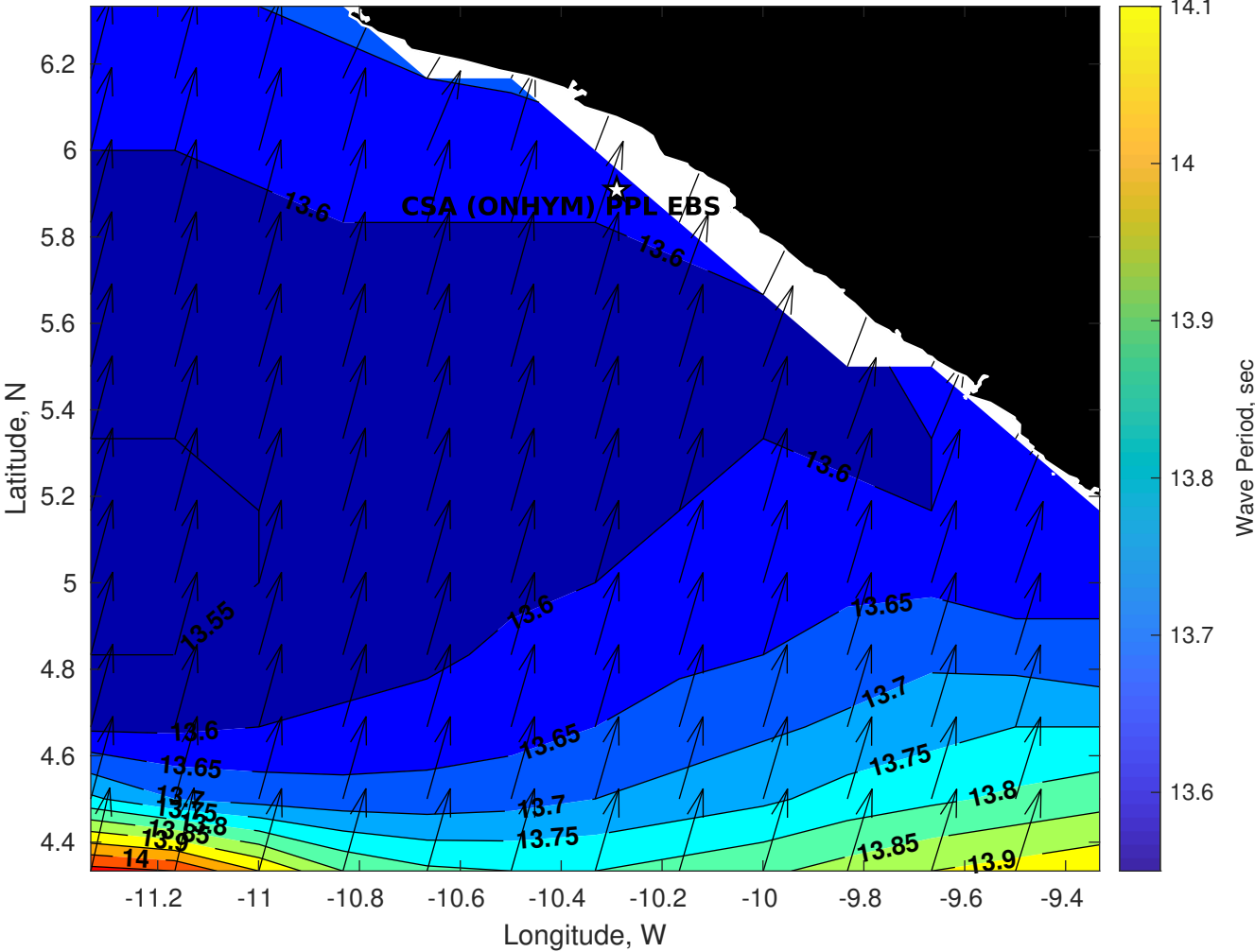
Wave Period (sec) for CSA (ONHYM) PPL EBS - Liberia at 19-May-2025 09:00:00
