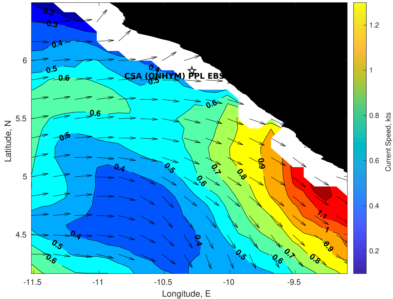
Surface Currents for CSA (ONHYM) PPL EBS - Liberia at 18-May-2025 00:00:00
