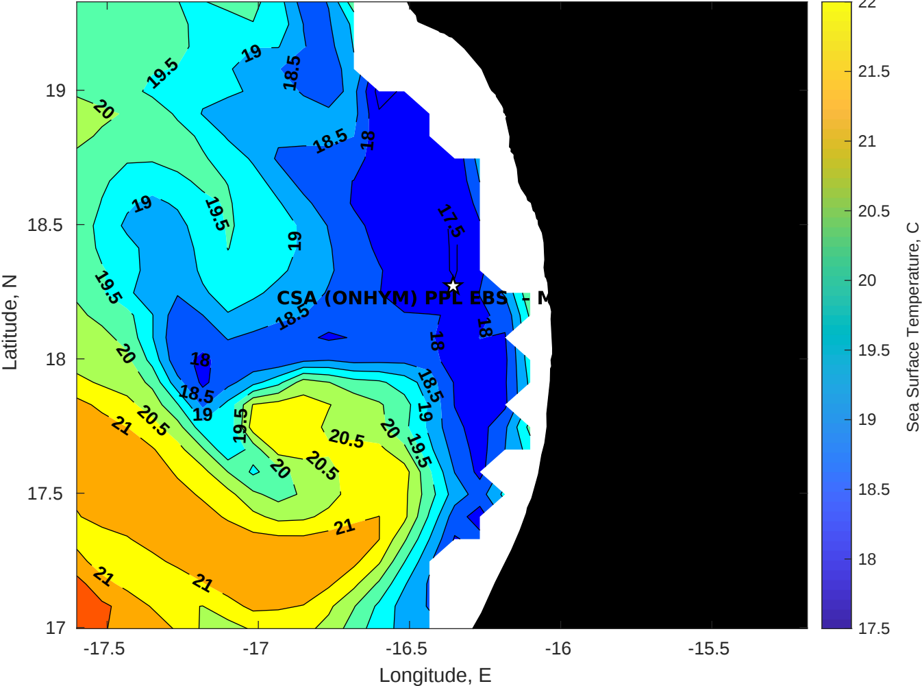
SST for CSA (ONHYM) PPL EBS - Mauritania at 18-May-2025 00:00:00
