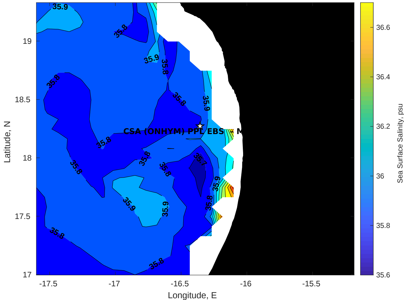
Surface Salinity for CSA (ONHYM) PPL EBS - Mauritania at 18-May-2025 00:00:00
