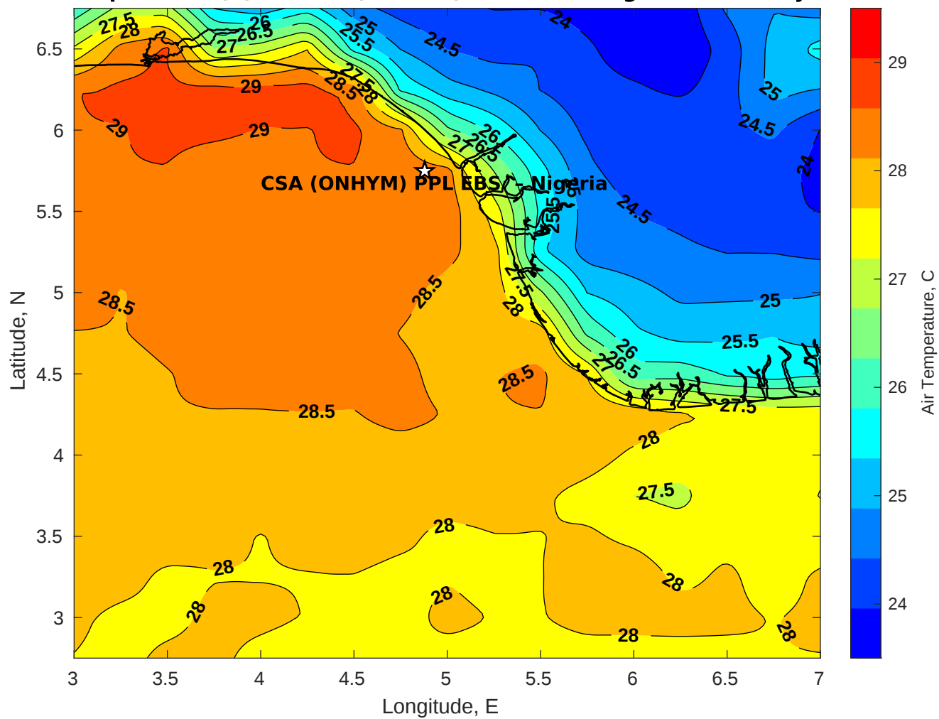
Air Temperature (C) for CSA (ONHYM) PPL EBS - Nigeria at 19-May-2025
