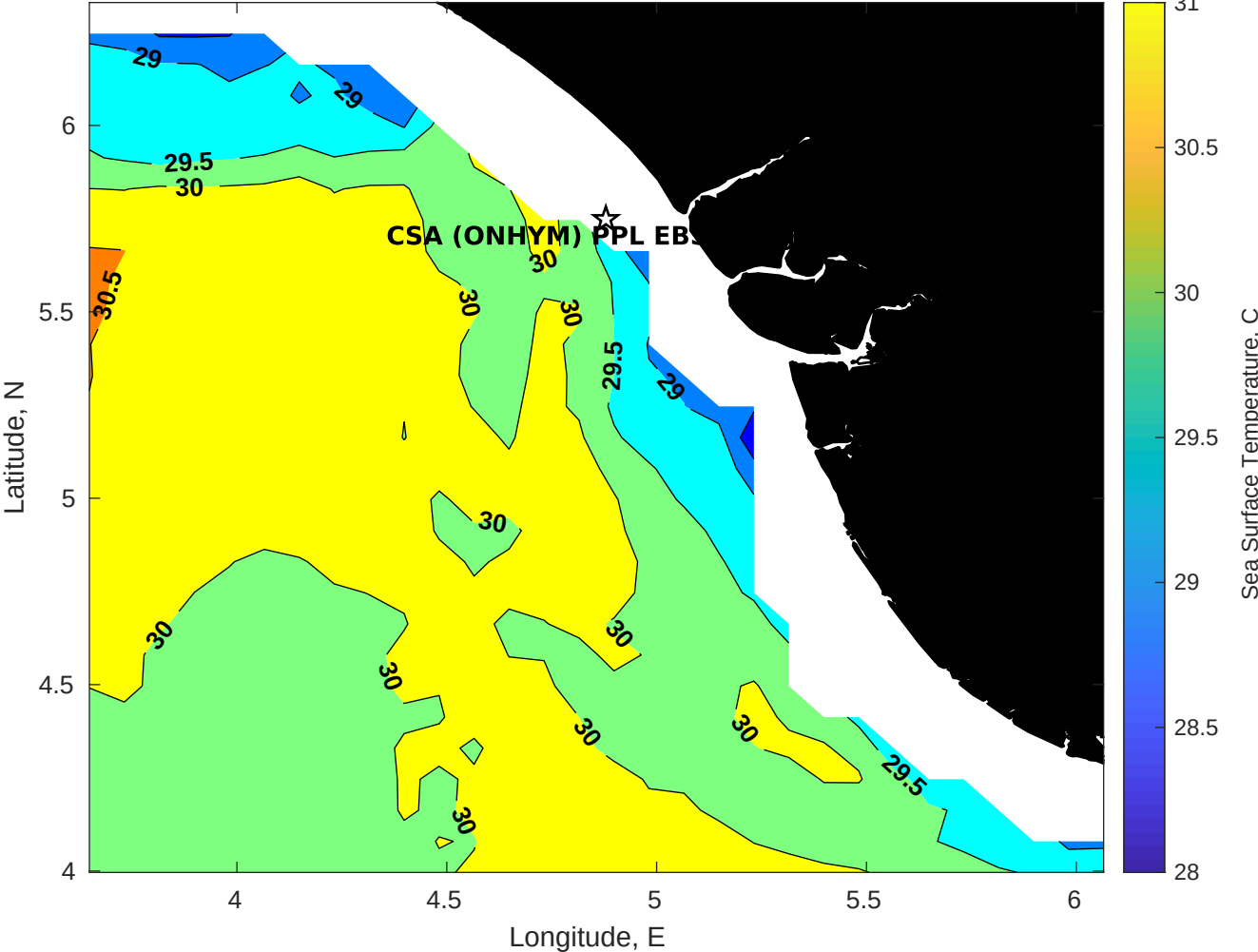
SST for CSA (ONHYM) PPL EBS - Nigeria at 18-May-2025 00:00:00
