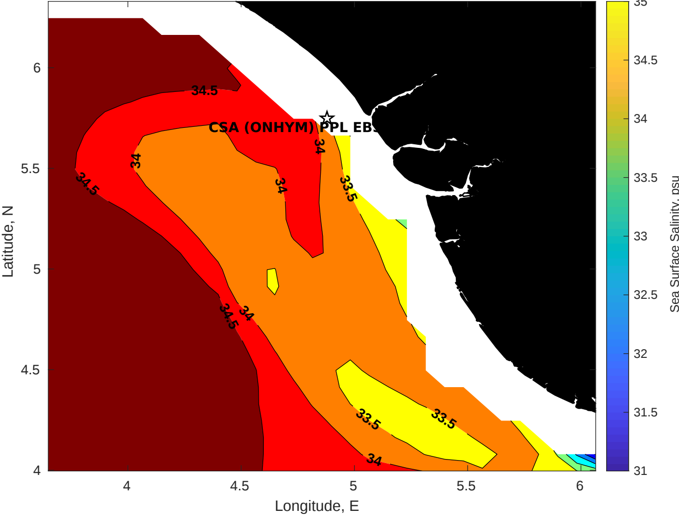
Surface Salinity for CSA (ONHYM) PPL EBS - Nigeria at 18-May-2025 00:00:00
