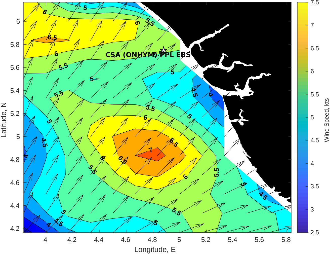
Winds (kts) for CSA (ONHYM) PPL EBS - Nigeria at 19-May-2025 09:00:00
