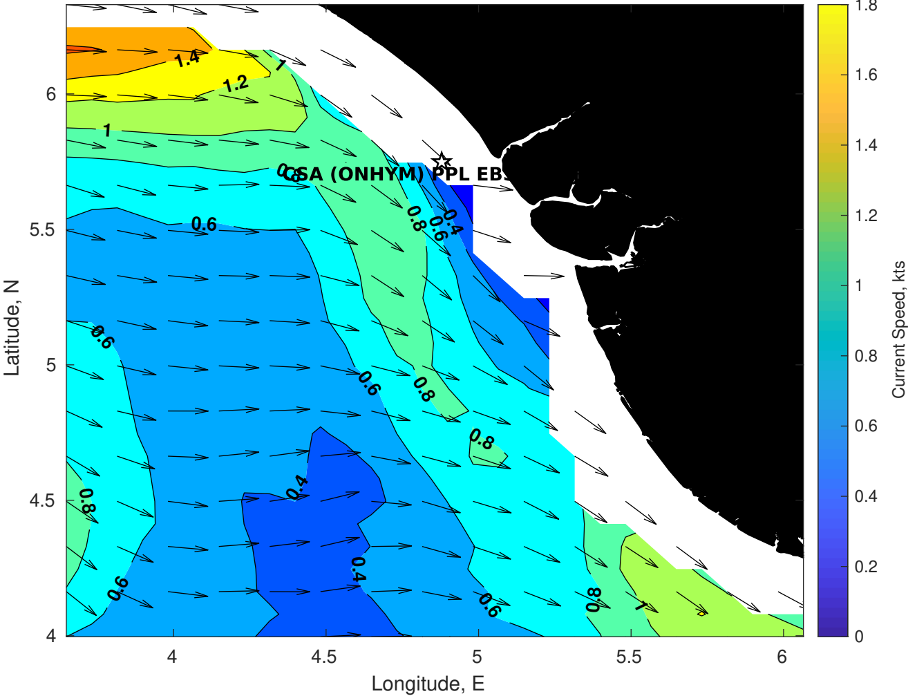
Surface Currents for CSA (ONHYM) PPL EBS - Nigeria at 18-May-2025 00:00:00
