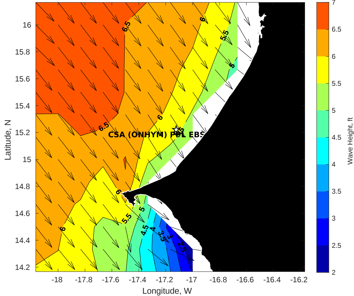
Wave Height (ft) for CSA (ONHYM) PPL EBS - Senegal at 19-May-2025 09:00:00
