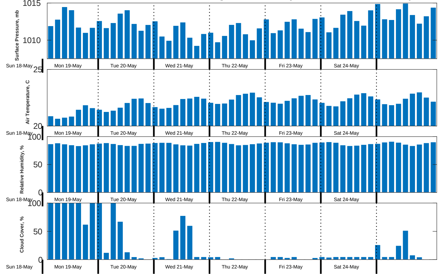
Met Forecast for CSA (ONHYM) PPL EBS - Senegal from 19-May-2025 00:00:00 to 26-May-2025 00:00:00
