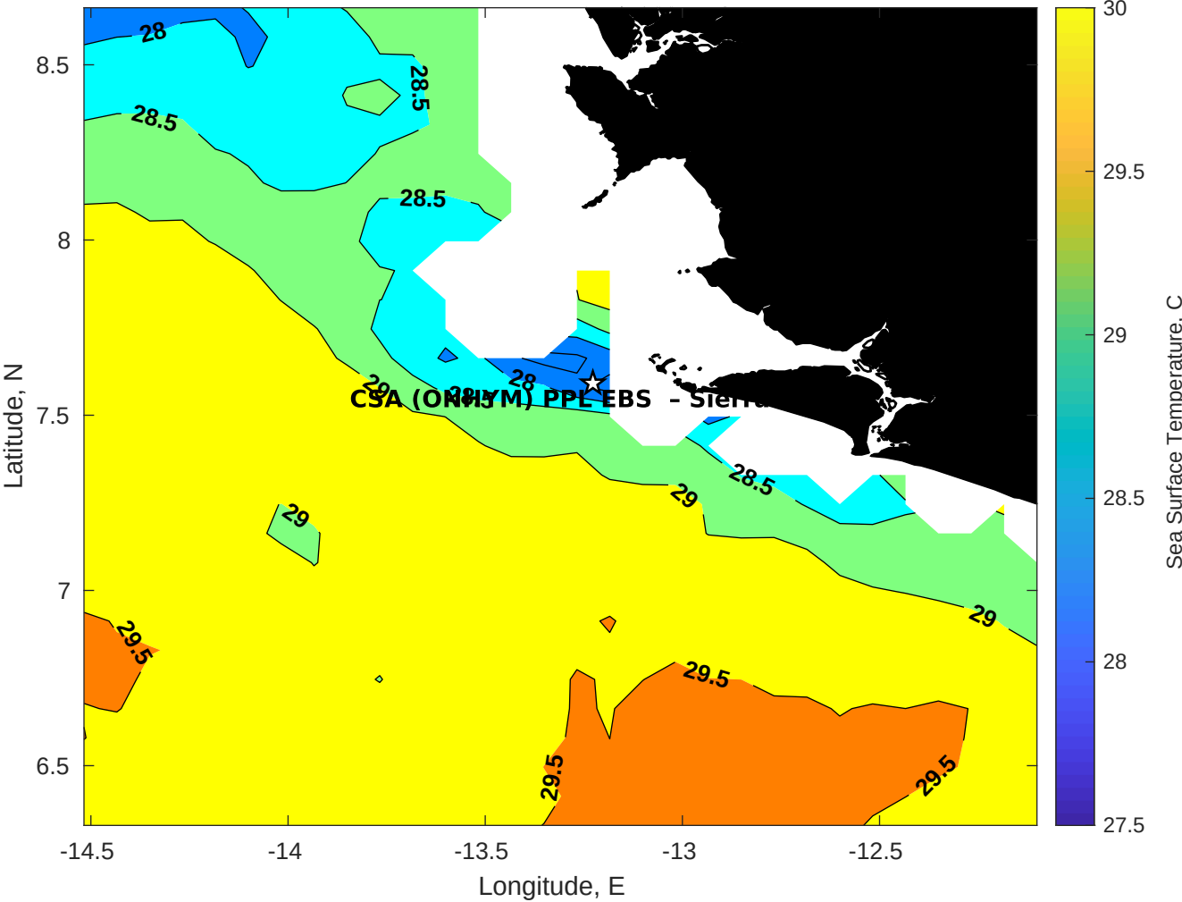
SST for CSA (ONHYM) PPL EBS - Sierra Leone at 18-May-2025 00:00:00
