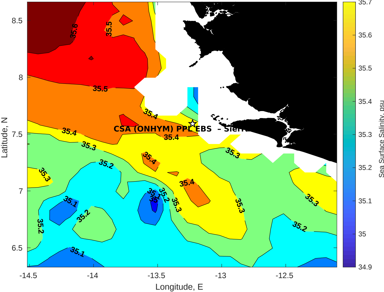
Surface Salinity for CSA (ONHYM) PPL EBS - Sierra Leone at 18-May-2025 00:00:00
