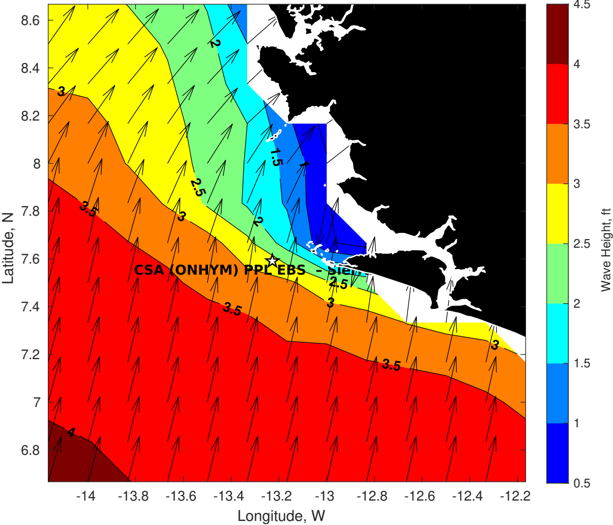
Wave Height (ft) for CSA (ONHYM) PPL EBS - Sierra Leone at 19-May-2025 09:00:00
