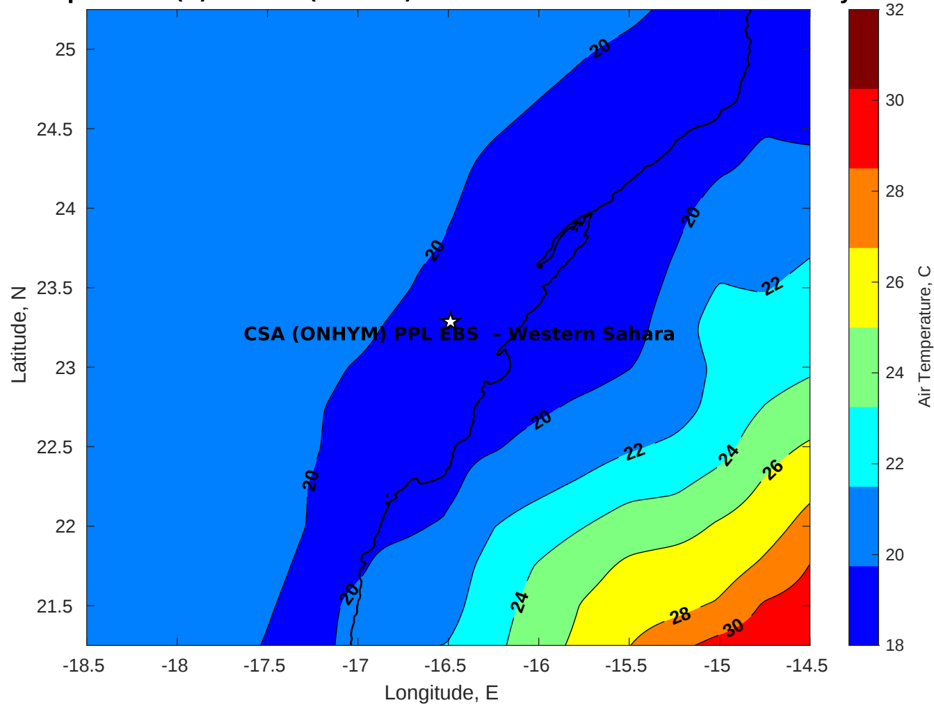
Air Temperature (C) for CSA (ONHYM) PPL EBS - Western Sahara at 19-May-2025
